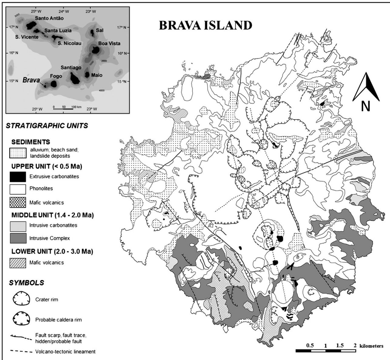
Fig. 1. Location of Brava in Cape Verde archipelago (inset) and geological sketch representing main stratigraphic units and structures. Simplified from Madeira et al. (2010).
