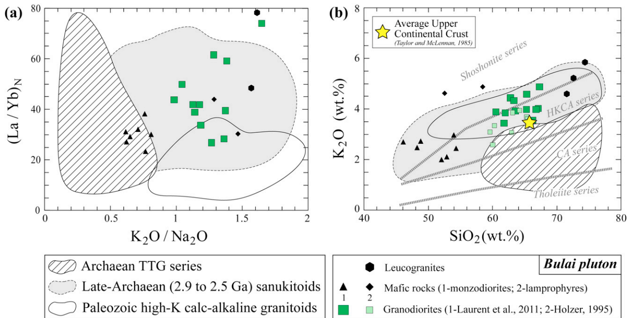
Fig. 1. Comparison between the compositions of Archean TTGs, late-Archaean sanukitoids and modern (Palaeozoic) high-K calc-alkaline granitoids. Samples from the Bulai pluton, which is the focus of this study, are also plotted and fall within the field of late-Archaean sanukitoids. (a) REE fractionation (expressed as La/Yb ratio normalized to chondritic value from McDonough and Sun, 1995) plotted vs. K_2O/Na_2O ratio. (b) Harker plot for K_2O , labeled with differentiation series as defined by Peccerillo and Taylor (1976). Note that the sanukitoid field (and samples from the Bulai pluton) straddles the boundary between high-K calc-alkaline and shoshonite series. Data for TTGs, sanukitoids and Palaeozoic granitoids are from author's databases (available on request).
