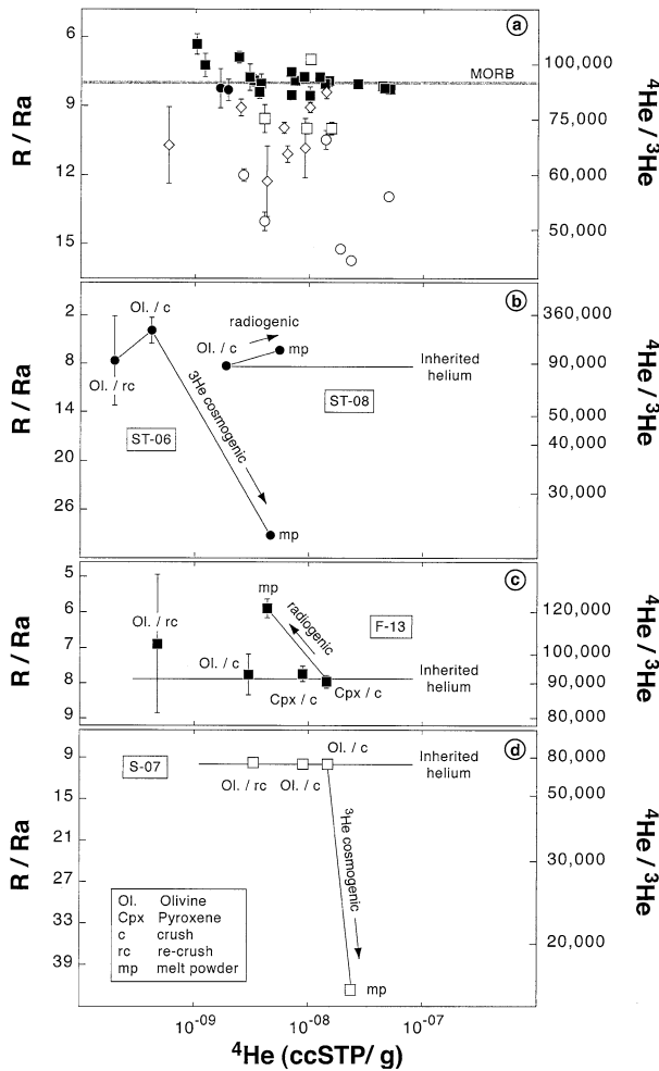
Fig. 7. Diagrams of R/R_A (and absolute {}^4\text{He}/{}^3\text{He} ) ratios vs. {}^4\text{He} concentrations for studied Cape Verde basalts. (a) Results for all olivine and pyroxene separates from samples analyzed using the crushing protocol compared to the MORB reference composition; symbols as in Figure 6. (b-d) Results for olivines and pyroxenes from samples ST-06, ST-08, F-13 and S-07; key to symbols and analytical steps in (d). The crushing of olivines and pyroxenes from samples F-13 and S-07 yields similar R/R_A ratios. This implies that the {}^4\text{He}/{}^3\text{He} ratios obtained by crushing are representative of the magmatic values (inherited helium). Melt products (mp) indicate that excesses of radiogenic {}^4\text{He} and cosmogenic {}^3\text{He} are present in the samples.
