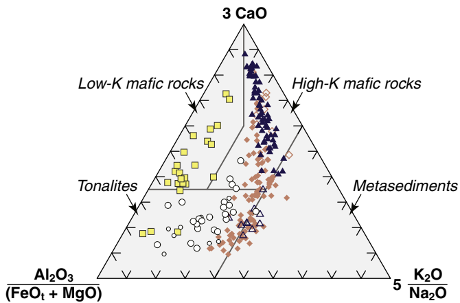
Fig. 6. Ternary diagram \text{Al}_2\text{O}_3/(\text{FeO}_t + \text{MgO}); 3 * \text{CaO}; 5 * (\text{K}_2\text{O}/\text{Na}_2\text{O}) on which the composition of late-Archean granitoids from the Pietersburg block and Limpopo Belt is plotted (symbols as in Figs. 4 and 5). The multiplication factors were only added for scaling purposes. The fields represent the composition of melts derived from a range of potential sources (tonalites, metasediments, low- and high-K mafic rocks), determined using the major-element compositions of experimental studies: Patiño-Douce and Beard (1995), Singh and Johannes (1996), Skjerlie and Johnston (1996), Watkins et al. (2007) for tonalites; Patiño-Douce and Beard (1996), Patiño-Douce and Johnston (1991), Vielzeuf and Holloway (1988) for metasediments; Beard and Lofgren (1991), Rapp et al. (1999), Rapp and Watson (1995), Wolf and Wyllie (1994) for low-K mafic rocks and Sisson et al. (2005) for high-K mafic rocks.
