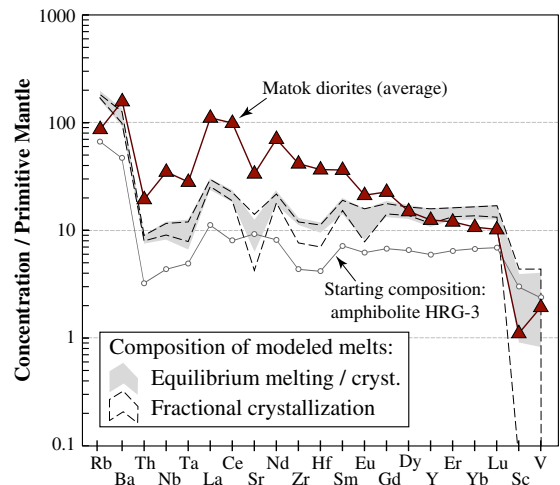
Fig. 9. Multi-element diagram with concentrations normalized to primitive mantle (McDonough and Sun, 1995) where the average trace element composition of the Matok diorites are compared to that of liquids derived from fractionation of tholeiitic amphibolites from the northern Kaapvaal craton. The latter were calculated using either the batch melting equation C_0 = C_1 \cdot [F + D \cdot (1 - F)] of Shaw (1976) for both equilibrium melting and equilibrium crystallization or the Rayleigh equation C_0 = C_1 / F^{D-1} for fractional crystallization. The starting composition is represented by amphibolite sample HRG-3 (major- and trace element composition reported in Supplementary Material). Fractionating minerals (60% plagioclase + 20% clinopyroxene + 10% orthopyroxene + 8% ilmenite + 2% magnetite) as well as the mass fraction of liquid ( F = 0.35 ) were derived from experimental run HG385 of Tatsumi and Suzuki (2009). The result of the model is a range of possible compositions, rather than a unique value, because we used a range of possible partition coefficients (Kd) from a minimum value to a maximum one (see Table 3 in Laurent et al., 2013a for details and values).
