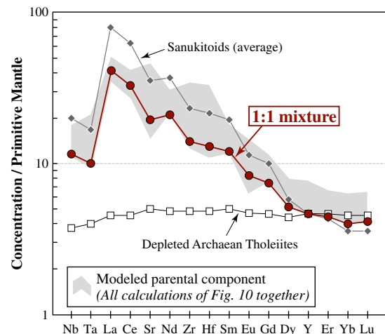
Fig. 13. Multi-element diagram for “immobile” elements with concentrations normalized to primitive mantle (McDonough and Sun, 1995) showing the results of binary mixing model (1:1) between average composition of sanukitoids (Martin et al., 2009; gray diamonds) and that of depleted Archean tholeiites (Condie, 1981; white squares). The trace element patterns and concentrations of the calculated mixture (red circles) reasonably match those of the calculated parental component of the Matok diorites.
