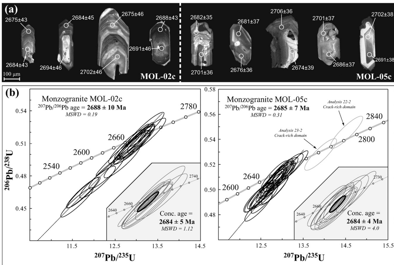
Fig. 6. (a) CL pictures of selected zircon grains from samples of the Moletsi pluton. The circles represent the position of laser spots used for age determination, and the associated values are the resulting ^{207}\text{Pb}/^{206}\text{Pb} age (in Ma) and its uncertainty ( 2\sigma ). (b) Concordia plots ( ^{206}\text{Pb}/^{238}\text{U} vs. ^{207}\text{Pb}/^{235}\text{U} ) for data obtained on samples from the Moletsi pluton. Light gray ellipses represent analyses that were not used to calculate the ^{207}\text{Pb}/^{206}\text{Pb} age. The insert on the bottom right is a close-up on the Concordia showing the analyses used for the calculation of the Concordia (Conc.) age. Error ellipses are 2\sigma .
