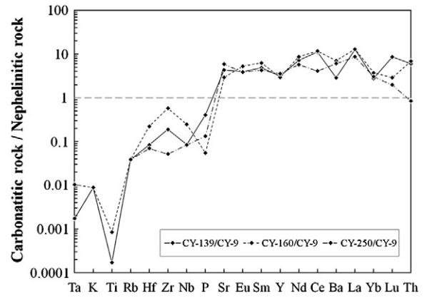
Fig. 12. Enrichment/depletion factors for selected elements of representative intrusive calcicarbonatites with respect to the composition of a nephelinitic rock from the Lower Unit (sample CY-9), plotting closest to the solvus and to the end of the tie line drawn in Fig. 11. The elements are arranged taking into account the experimental partition coefficients during silicate-carbonatite immiscibility processes (Hamilton et al., 1989; Veksler et al., 1998).
