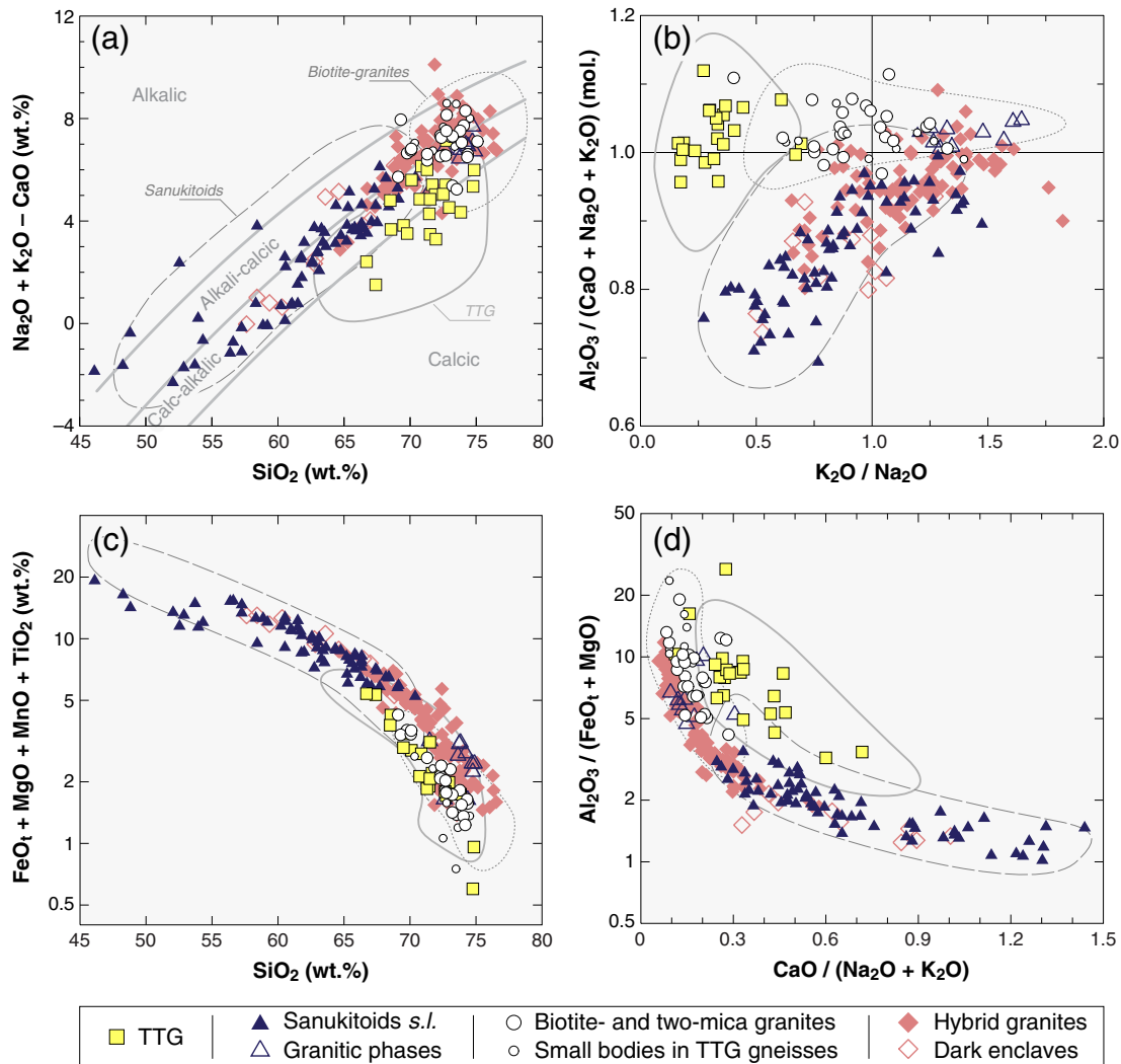
Fig. 4. Major-element geochemistry of the four groups of late-Archaean granitoids, illustrated with examples from the Pietersburg block and the Limpopo Belt (symbols) as well as literature data (fields; compilations from Martin et al., 2009; Moyen, 2011; Moyen and Martin, 2012). (a) MALI index [(\text{Na}_2\text{O} + \text{K}_2\text{O}) - \text{CaO}] vs. \text{SiO}_2 diagram of Frost et al. (2001); (b) A/CNK (molar \text{Al}_2\text{O}_3/[\text{CaO} + \text{Na}_2\text{O} + \text{K}_2\text{O}] ratio) vs. \text{K}_2\text{O}/\text{Na}_2\text{O} ratio; (c) sum of “mafic” oxides ( \text{FeO}_t + \text{MgO} + \text{MnO} + \text{TiO}_2 ) vs. \text{SiO}_2 ; and (d) \text{Al}_2\text{O}_3/(\text{FeO}_t + \text{MgO}) ratio vs. \text{CaO}/(\text{Na}_2\text{O} + \text{K}_2\text{O}) ratio.
