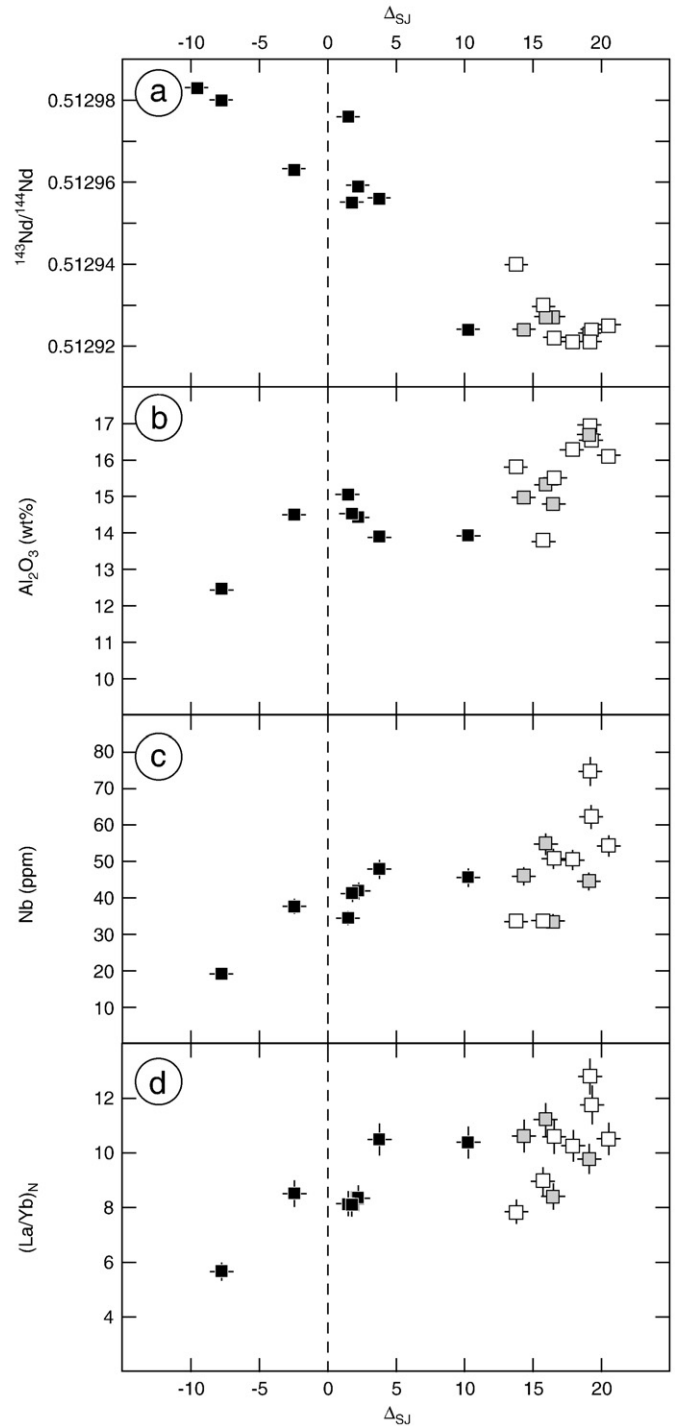
Fig. 10. Variations of major and trace element contents as well as major, trace element and isotope ratios with the \Delta_{Sj} parameter (see text for details). Co-variations recorded between (a) ^{143}\text{Nd}/^{144}\text{Nd} , (b) \text{MgO} , (c) \text{Al}_2\text{O}_3 , (d) (\text{La}/\text{Yb})_N and the \Delta_{Sj} parameter indicate that magmatic differentiation and mixing occurs simultaneously, mostly affecting Rosais and Manadas samples. The component responsible for isotopic variations is therefore most likely assimilated during an AFC process.
