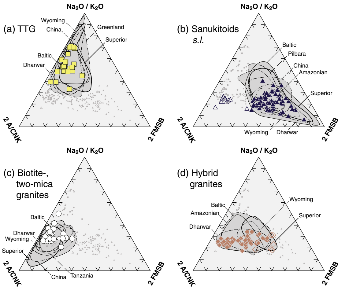
Fig. 7. Proposed ternary classification diagram for late-Archean granitoids: 2 * A/CNK (molar Al_2O_3/[CaO + Na_2O + K_2O] ratio); Na_2O/K_2O ratio; 2 * (FeO + MgO)_{wt\%} * (Sr + Ba)_{wt\%} (= FMSB). The multiplication factors were only added for scaling purposes. Examples of each group of late-Archean granitoids were plotted on the diagram, including samples from the Pietersburg block and the Limpopo Belt in South Africa (symbols) as well as 7 other cratons worldwide (for references, see Table 2). This diagram can be used as a petrogenetic indicator, each pole representing an end-member source of late-Archean granitoids: (1) pre-existing crustal rocks (pole A/CNK); (2) low-K mafic rocks (pole Na_2O/K_2O ); and (3) a LILE-rich, metasomatized mantle (pole FMSB). The hybrid granitoids plot in the convergence area of the other three groups. See text for details.
