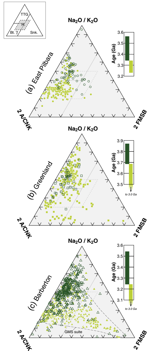
Fig. 14. Comparison of early Archean (>3.0 Ga-old) granitoids with the fields of late-Archean (3.0–2.5 Ga) granitoids (inset in the top left corner; Snk. = sanukitoids s.l., Bt. \gamma = biotite- and two-mica granites, H. = hybrids) in the synthetic classification diagram of Fig. 7 (see also Section 2.5). Early Archean data are from three different Paleo- to Mesoarchean terranes in which a secular evolution of granitoid compositions has been reported: (a) the East Pilbara Craton, NW Australia; (b) SW Greenland; (c) the area of the Barberton Greenstone Belt, South Africa. In a given area, granitoids are classified into two groups: (i) “early” granitoids (open dark green symbols) and (ii) “late” granitoids (filled light green symbols) on the basis of published models for crustal evolution in these terranes. The adjacent timelines indicate the approximate age range for each group. In (c), the dashed field encloses samples of the Granite–Monzogranite–Syenite (GMS) suite of the Barberton region. Data are from published or personal databases (Moyen, 2011; Moyen and Martin, 2012; J.F. Moyen).
