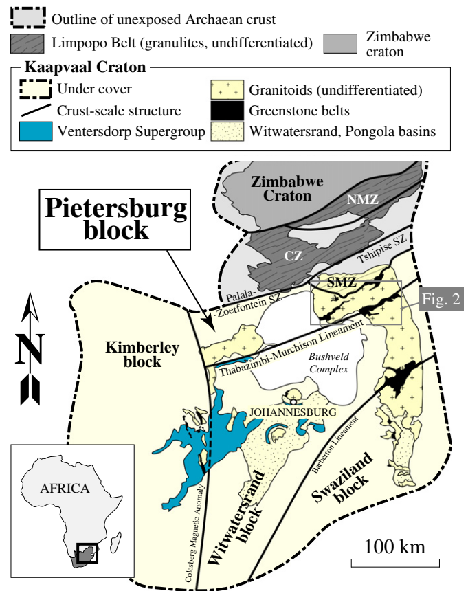
Fig. 1. Sketch of geological map (after Eglinton and Armstrong, 2004) detailing the different structural domains of the Kaapvaal craton. The position of the Pietersburg block and the Venterdorp supergroup are highlighted. The gray rectangle represents the study area. NMZ, CZ and SMZ refer to the three structural domains of the Limpopo Belt, i.e. Northern Marginal Zone, Central Zone and Southern Marginal Zone, respectively.
