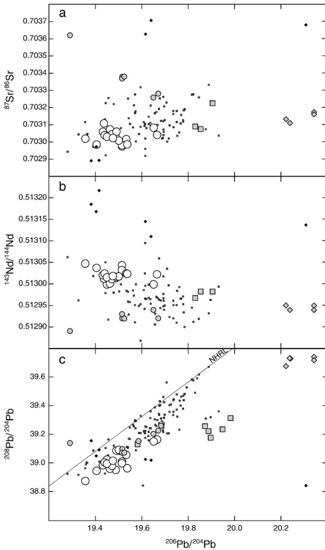
Fig. 6. Plot of ^{87}\text{Sr}/^{86}\text{Sr} (a), ^{143}\text{Nd}/^{144}\text{Nd} (b), ^{208}\text{Pb}/^{204}\text{Pb} (c) vs. ^{206}\text{Pb}/^{204}\text{Pb} isotopes ratios for São Nicolau samples. Symbols as in Fig. 5 and are bigger than errorbars. Most of our samples plot at ^{206}\text{Pb}/^{204}\text{Pb} < 19.6 , whereas two samples are plotting distinctly from this group, toward Fogo or São Vicente carbonatites (age-corrected data from Gerlach et al. (1988) and Hoernle et al. (2002)).
