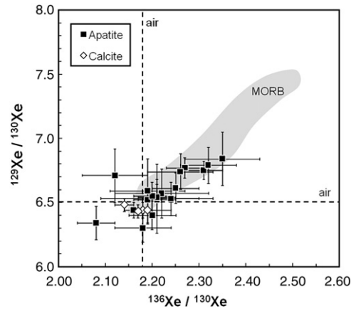
Fig. 4. ^{129}\text{Xe}/^{130}\text{Xe} vs. ^{136}\text{Xe}/^{130}\text{Xe} ratios. Carbonatite samples show ^{129}\text{Xe} and ^{136}\text{Xe} excesses when compared to air. These excesses reflect the presence of a mantle component that could be MORB- or OIB-derived. Only samples with blanks lower than 15% of the measured xenon are reported.
