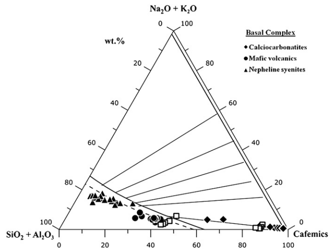
Fig. 11. Projection of rock compositions from the Basal Complex in the (\text{SiO}_2 + \text{Al}_2\text{O}_3) - (\text{Na}_2\text{O} + \text{K}_2\text{O}) - \text{Cafemics} ( \text{CaO} + \text{FeO} + \text{MgO} + \text{MnO} ) diagram; the topology of the carbonate-silicate liquid immiscibility experimental system (Kjarsgaard and Hamilton, 1988) is also presented. Open squares are the compositions of carbonate- and silicate-rich conjugate melts from Dasgupta et al. (2006). The solvus at 0.5 GPa (bold continuous line) and at 0.8 GPa (dashed line) as well as the experimentally determined tie-lines for different carbonatite-silicate conjugate liquids are shown. This diagram supports the occurrence of an immiscibility process to explain the origin of calcicarbonatites from the Basal complex. For comparison with extrusive silicate and carbonatite rocks from the Upper Unit, see Fig. 11 in Mourão et al. (2010). The composition of some nephelinites can be observed to have conjugate carbonatitic liquids plotting very close to the Cafemic corner.
