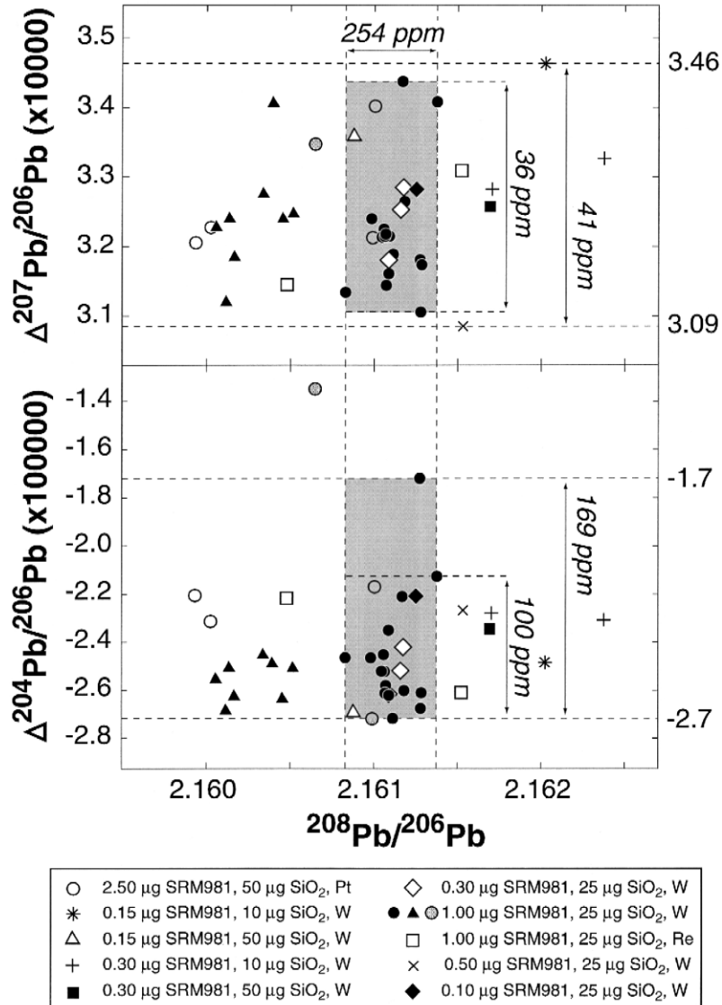
Fig. 4. External reproducibilities of ^{207}\text{Pb}/^{206}\text{Pb} and ^{204}\text{Pb}/^{206}\text{Pb} ratios. Black and grey circles are for 1 \times 10^{-6} g Pb spread loads; running temperature ranges between 1050°C and 1175°C for the first, and between 990 and 1010 for the second, respectively. Black triangles correspond to 1 \times 10^{-6} g Pb centered loads. For given amounts of lead and silica-gel, spread and centered loads show small distinct mass discrimination (around 1.8 \times 10^{-4} per amu) but similar reproducibilities.
