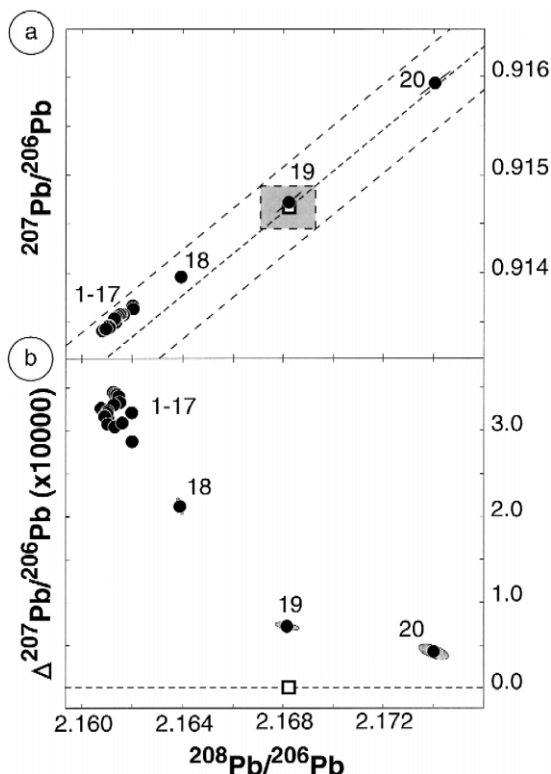
Fig. 1. Comparison of the ^{207}\text{Pb}/^{206}\text{Pb} and the ^{207}\text{Pb}/^{206}\text{Pb} vs. ^{208}\text{Pb}/^{206}\text{Pb} diagrams. A typical experiment with the SRM981 standard (Table 1) is shown. Each full dot plots a data block with its corresponding number. The uncertainty associated to each block is smaller than the symbol size, blocks 18 to 20 excepted. Open-square plots the nominal value of the SRM981 with its overall limit of error (Catanzaro et al., 1968). Dashed lines plot the mass discrimination lines through the certified value. The ^{207}\text{Pb}/^{206}\text{Pb} representation points out more clearly than the Pb–Pb diagram the small but significant scatter of the data set and the deviation of the mass discrimination from a linear evolution.
