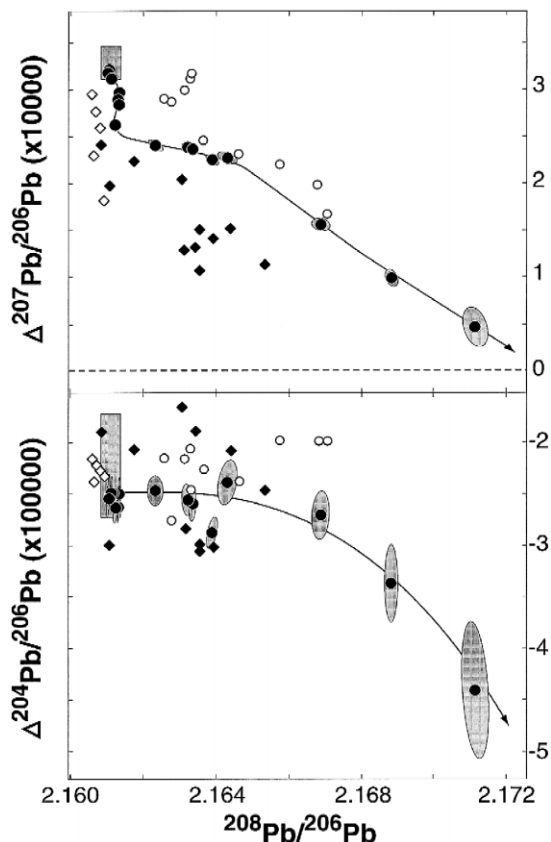
Fig. 7. Recent TIMS measurements with SRM981. Raw isotopic compositions (i.e. not corrected for mass discrimination) are plotted. Full circles along the dashed line show a typical isotopic evolution of this study. Rectangles show the domain of reproducibility of our first low temperature measurements. Open circles are for Thirlwall (2000), open diamonds for Woodhead et al. (1995) and black diamonds for Todt et al. (1996). The data of Woodhead et al. (1995) and Todt et al. (1996) are average run measurements. Each data set shows a nonlinear evolution in the \Delta^{207}\text{Pb}/^{206}\text{Pb} vs. ^{208}\text{Pb}/^{206}\text{Pb} plot. Previous data are coherent with our first data blocks in the \Delta^{204}\text{Pb}/^{206}\text{Pb} vs. ^{208}\text{Pb}/^{206}\text{Pb} diagram.
