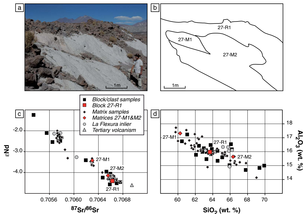
Figure 8. (a) Photograph, (b) schematic field relationship, (c) \epsilon\text{Nd} versus ^{87}\text{Sr}/^{86}\text{Sr} , and (d) \text{Al}_2\text{O}_3 versus \text{SiO}_2 diagrams for samples from outcrop 27 (see Figure 2 for location). The southwest edge of the proximal zone of the avalanche shows complex relationships between matrices and blocks in contact compared to the central part where both types of samples have identical isotope ratios.
