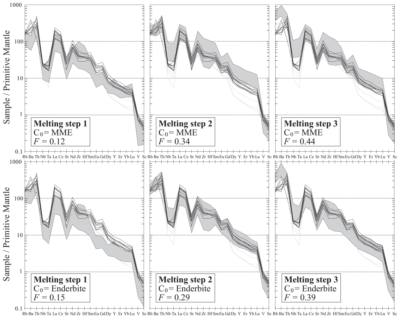
Fig. 10. Primitive mantle-normalized trace-element patterns for the Bulai granodiorites (black patterns) as well as Monte-Carlo models of partial melting following the melting sequence described in Section 4.4. Models were tested for source rocks represented by MME and enderbites (upper and lower part, respectively). The grey field represents the compositional range of computed liquids with the melting rate ( F ) indicated in the caption for the three successive melting steps (see Table 6 and text for explanation). The light grey patterns represent the compositions of samples BUL-16, BUL-22 and BUL-23. Note that the best fit is obtained for the Step 2 of enderbite melting.
