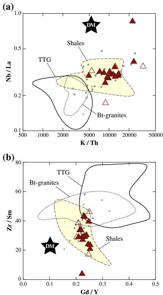
Fig. 11. Plots of selected minor- and trace element ratios that are not significantly fractionated during mantle melting and differentiation of mafic melts: (a) Nb/La vs. K_{ppm}/Th and (b) Zr/Sm vs. Gd/Y. The Matok diorites are represented by red triangles, granodiorites by gray circles and monzogranites by gray diamonds. The composition of the diorites overlap that of detrital sedimentary rocks from the Pietersburg block (data from Kreissig et al., 2000) for both diagrams, while minor- and trace element ratios in TTGs (data from Kreissig et al., 2000; Kröner et al., 2000; Laurent et al., in revision) and biotite-bearing granites (data from Henderson et al., 2000; Kröner et al., 2000; Laurent et al., in revision) are different.
