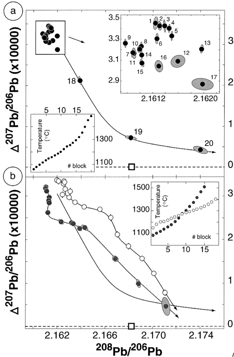
Fig. 2. Experiments with the SRM981 standard. (a) These are the measurements of the experiment compiled in Table 1. Numbers refer to data blocks, ellipses show the uncertainties. The inset on the right highlights the isotopic evolution from block 1 to 17. The inset on the left shows the step heating (Table 1) to maintain the ^{204}\text{Pb} beam at around 2 \times 10^{-12} A. The dashed line plots the linear mass discrimination passing through the nominal value of the SRM981 standard (open square). The last data blocks (18 to 20) display the most important shifts, but a deviation from the linear evolution appears from block 5 after about 2 h of heating. (b) This shows distinct evolutions observed for three similar experiments ( 1 \times 10^{-6} g Pb, spread loads). The dashed line without any symbol corresponds to the experiment plotted in (a). The isotopic evolution mostly depends on the heating conditions (inset).
