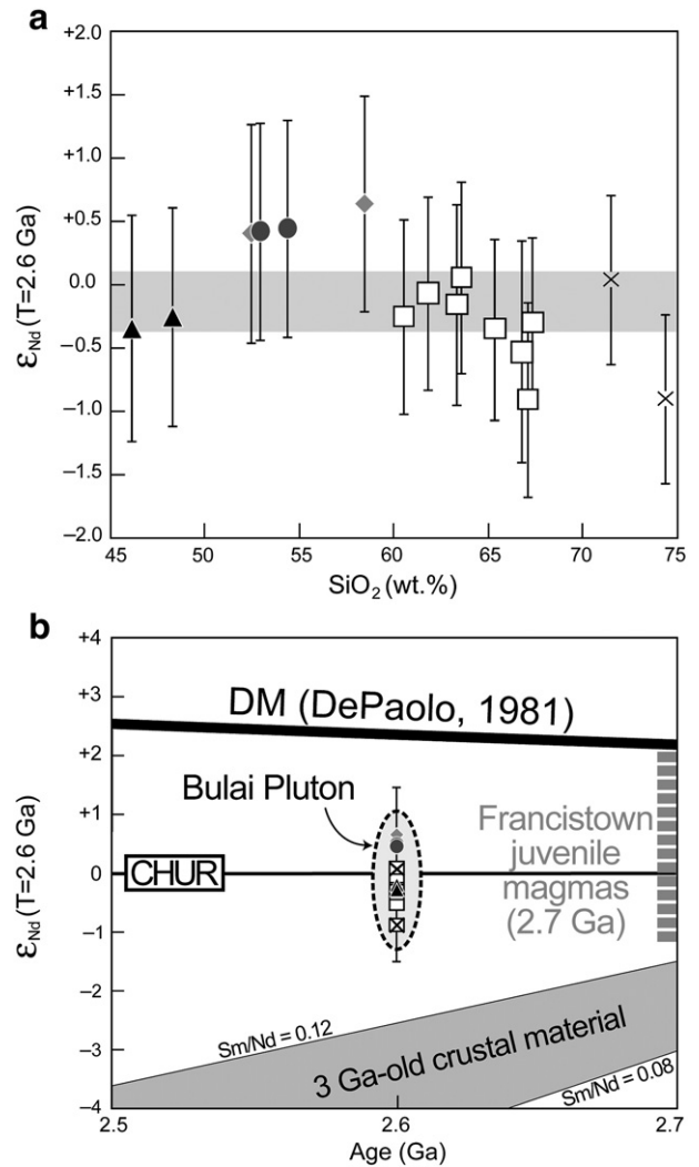
Fig. 9. ^{143}Nd/^{144}Nd initial isotopic compositions of the Bulai rocks. (a) \epsilon_{Nd}(T=2.6 Ga) vs. SiO_2 diagram showing the “juvenile” character ( -1.5 < \epsilon_{Nd} < +1.5 ) of all the rocks from the Bulai suite, regardless of their silica content. The error bars are 2\sigma uncertainty and the grey field represents the weighted average of all analyses. (b) Plot of \epsilon_{Nd} vs. age. The isotopic signature of the Bulai samples is similar to the one of the Francistown juvenile TTGs and sanukitoids (Zhai et al., 2006), and far from the one of a virtual “pristine” crustal component extracted from the DM at 3 Ga (light grey field). Symbols are as in Fig. 6.
