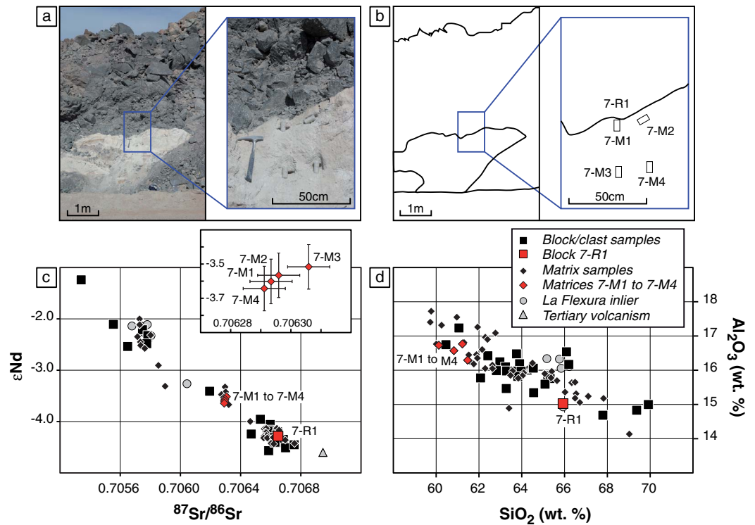
Figure 4. (a) Photograph, (b) schematic field relationship, (c) \epsilon Nd versus ^{87}\text{Sr}/^{86}\text{Sr} , and (d) \text{Al}_2\text{O}_3 versus \text{SiO}_2 diagrams for samples from outcrop 7 (distal zone of the avalanche, see Figure 2 for exact location). The four matrix samples, 7-M1 to 7-M4, show only minor isotope and major element variations that can be considered as insignificant with respect to analytical uncertainties and reproducibilities. Block sample at contact (7-R1), however, presents significantly distinct isotopic and chemical signatures. Note the ingestion of the lava into the matrix (left of the caption).
