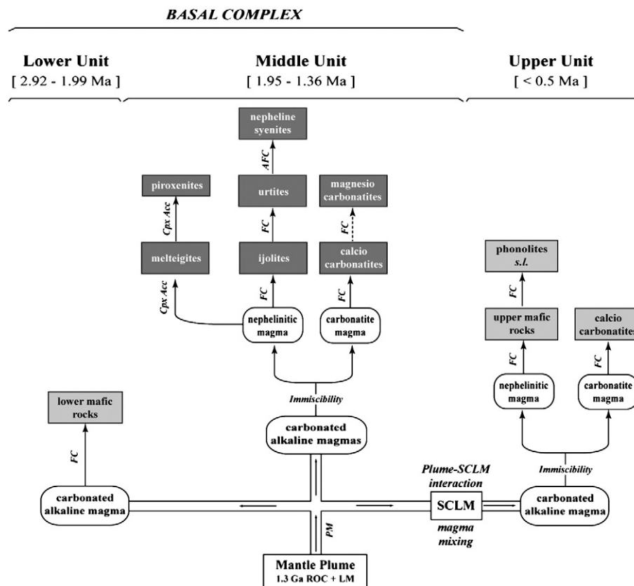
Fig. 13. Schematic illustration of the proposed scenario for the genesis and evolution of magmas at the origin of the three Brava Island volcanostratigraphic units. The “lower” and “upper” mafic volcanics include nephelinites, melilite nephelinites, basanites, foidites, tephrites and phonotephrites. The “phonolites s.l.” include phonolites and nepheline phonolites. PM, FC, Acc and AFC stand for Partial Melting, Fractional Crystallization, Accumulation and Assimilation and Fractional Crystallization processes, respectively. SCLM, subcontinental lithospheric mantle; ROC, ancient recycled oceanic crust; LM, lower mantle; Cpx, clinopyroxene; Cal, calcite. Dark gray boxes: intrusive rocks; light gray boxes: extrusive rocks. As shown, even though magnesio carbonatites of the Middle Unit are considered representative of a liquid residue left after calcite accumulation, they cannot be considered strictly comagmatic with the outcropping calcio carbonatites.
