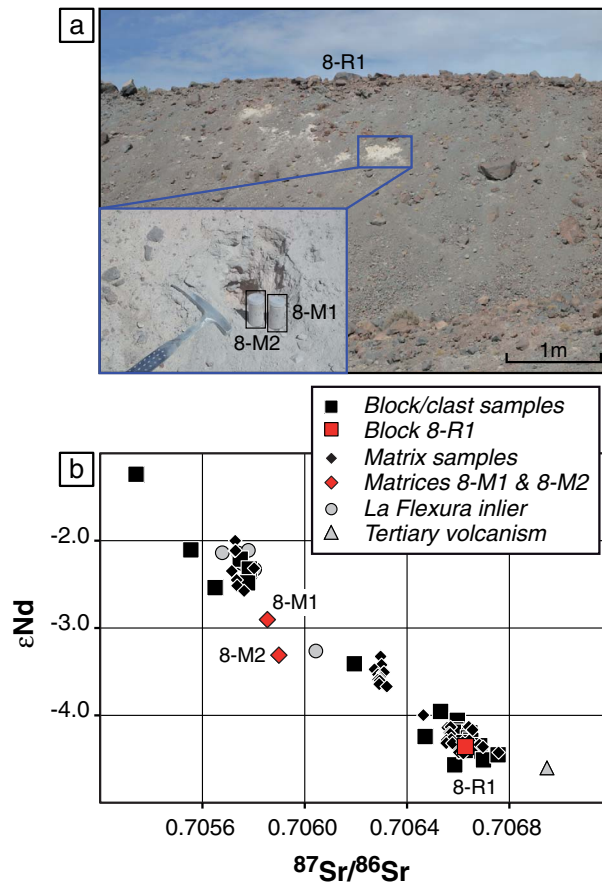
Figure 9. (a) Photograph and (b) \epsilon\text{Nd} versus ^{87}\text{Sr}/^{86}\text{Sr} diagram for samples from outcrop 8 (distal zone of the avalanche, see Figure 2 for exact location). Note there is only a thin, \sim 50 cm, layer of fragmented rocks, here represented by sample 8-R1, over a thick—more than a few meters—layer of matrix (samples 8-M1 and 8-M2). As for outcrop 7, matrices and block in contact present significantly distinct isotopic signatures.
