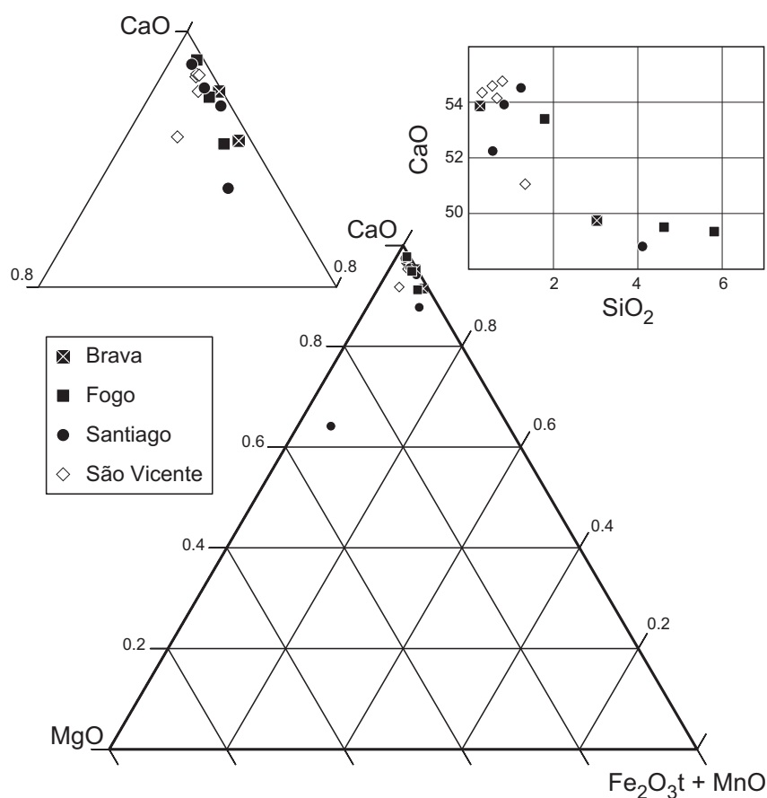
Fig. 2. Plot of Cape Verde carbonatites in terms of CaO–MgO–( Fe_2O_3 + MnO) together with CaO vs. SiO_2 . All samples but one are calcio-carbonatites. The broad negative trend between CaO and SiO_2 suggests either mechanical mixing between a pure carbonate end-member with CaO = 56 wt.% and silicates entrained during ascent, or traces of silicates dissolved in carbonate during partial melting.
