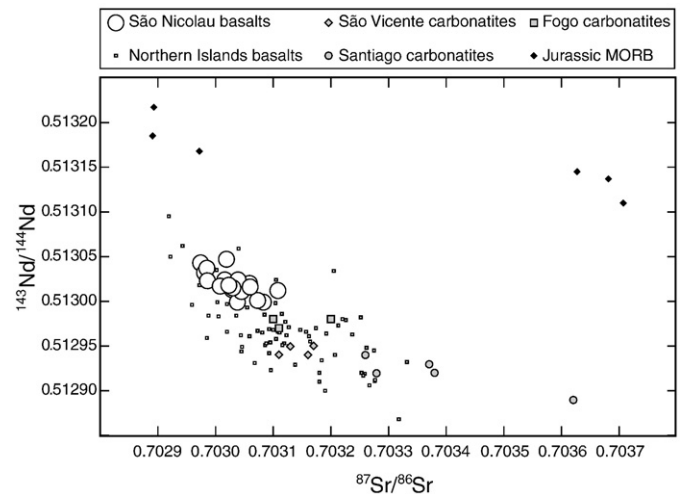
Fig. 5. ^{143}\text{Nd}/^{144}\text{Nd} vs. ^{87}\text{Sr}/^{86}\text{Sr} diagram for some Cape Verde volcanics. São Nicolau data: this study; Northern Islands (São Vicente, Santo Antão): (Gerlach et al., 1988; Christensen et al., 2001; Jørgensen and Holm, 2002; Doucelance et al., 2003; Holm et al., 2006), Jurassic MORB: Gerlach et al. (1988) and this study; Carbonatites: Gerlach et al. (1988), Hoernle et al. (2002). Samples from the São Nicolau Island plot within the Northern Island field, and have amongst the depleted values of this group of islands.
