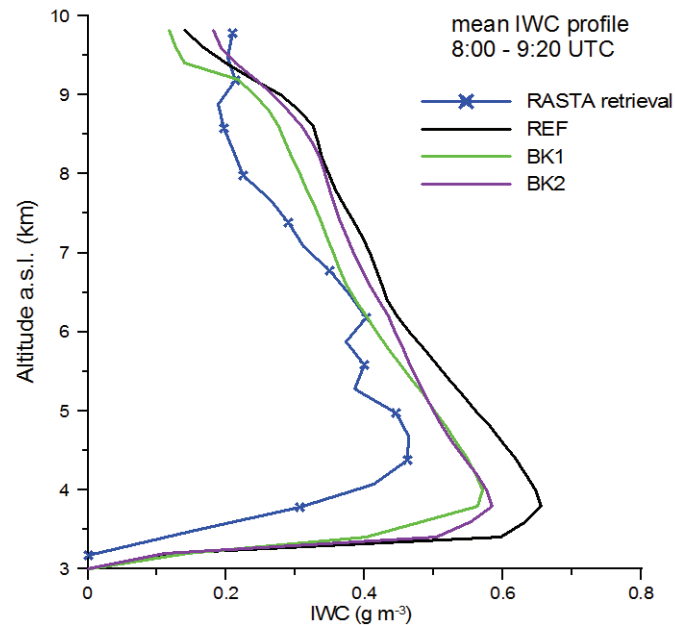
Figure 5.16: Time-averaged mean vertical profile of IWC (in \text{g m}^{-3} ) in the time period 8:00 UTC – 9:20 UTC for simulations REF, BK1 and BK2 together with the RASTA retrieval.
