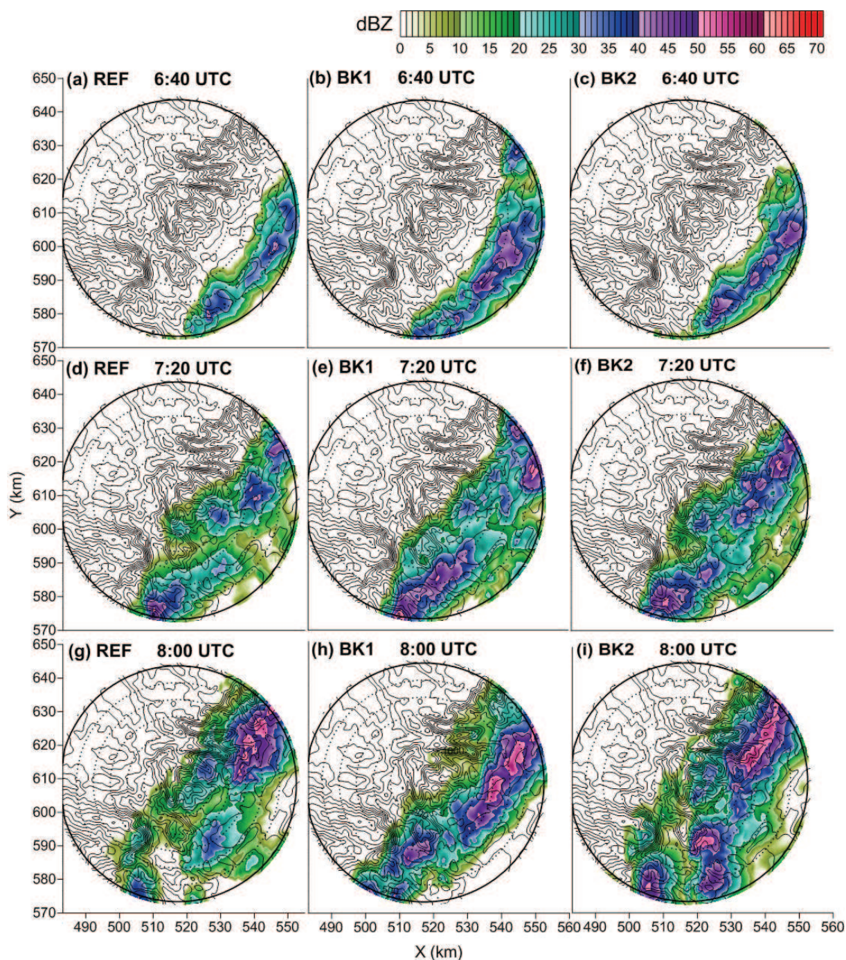
Figure 5.13: PPI images of the modeled radar reflectivity for the reference case (REF) at (a) 6:40 UTC, (d) 7:20 UTC and (g) 8:00 UTC, the simulation BK1 (b, e and h) and the simulation BK2 (c, f and i) at the same specific times. The solid black lines represent the topography and the concentric circles correspond to the different altitudes of the radar beam at every 5 km to the radar position. The maximum height of the radar beam (external circle in bold black) is 1892 m.
