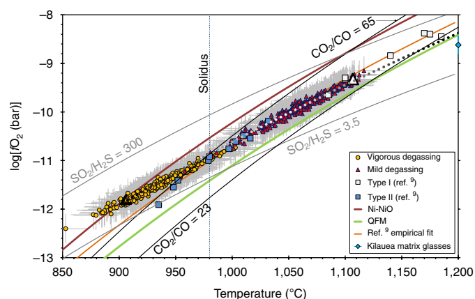
Fig. 3 | Computed equilibrium temperature and fO_2 for spectroscopic measurements of gas emissions from Kilauea's lava lake. The dataset is classified into mild-degassing (12:14 to 13:14 h local time) and vigorous-degassing (15:16 to 15:23 h) regimes on 5 March 2013. Also shown are NNO and QFM buffers; the solidus temperature of Kilauea basalt; computed ranges for given values of CO_2/CO and SO_2/H_2S ; temperature- fO_2 calculations for 'type I' and 'type II' gases (Kilauea Summit and East Rift Zone emissions, respectively) and associated empirical fit 9 ; and reported fO_2 at 1,200 °C for 2008 and 2010 matrix glasses for ejecta from Halema'uma'u Crater (mean and range shown) 29 . Note that, below the solidus, our analyses for 'vigorous degassing' are more oxidized than 'type II' gases at equivalent equilibrium temperatures. The white and black dotted line with arrow shows temperature- fO_2 calculations for closed-system, gas-only cooling starting with our measured gas composition at 1,150 °C (open triangle), showing a close fit to the dataset.
