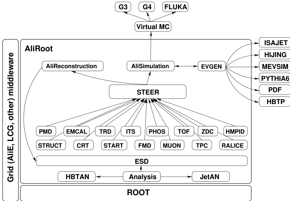
Figure 2.3: Schematic view of the AliRoot framework.
