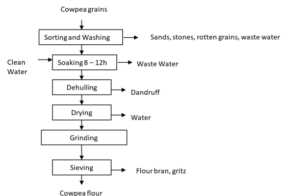
Figure 2: Process production of cowpea flour
