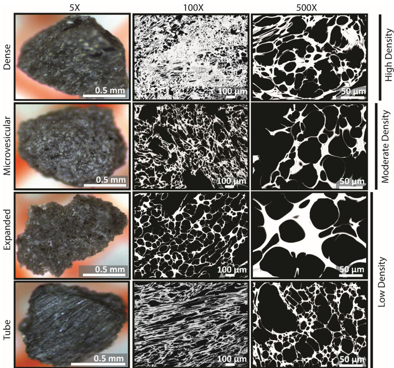
Fig. 6 Selected images of various types of pumice clasts taken by stereo-microscope and SEM at different magnifications (5×, 100×, and 500×). The pumice clasts are representative of the different clast
