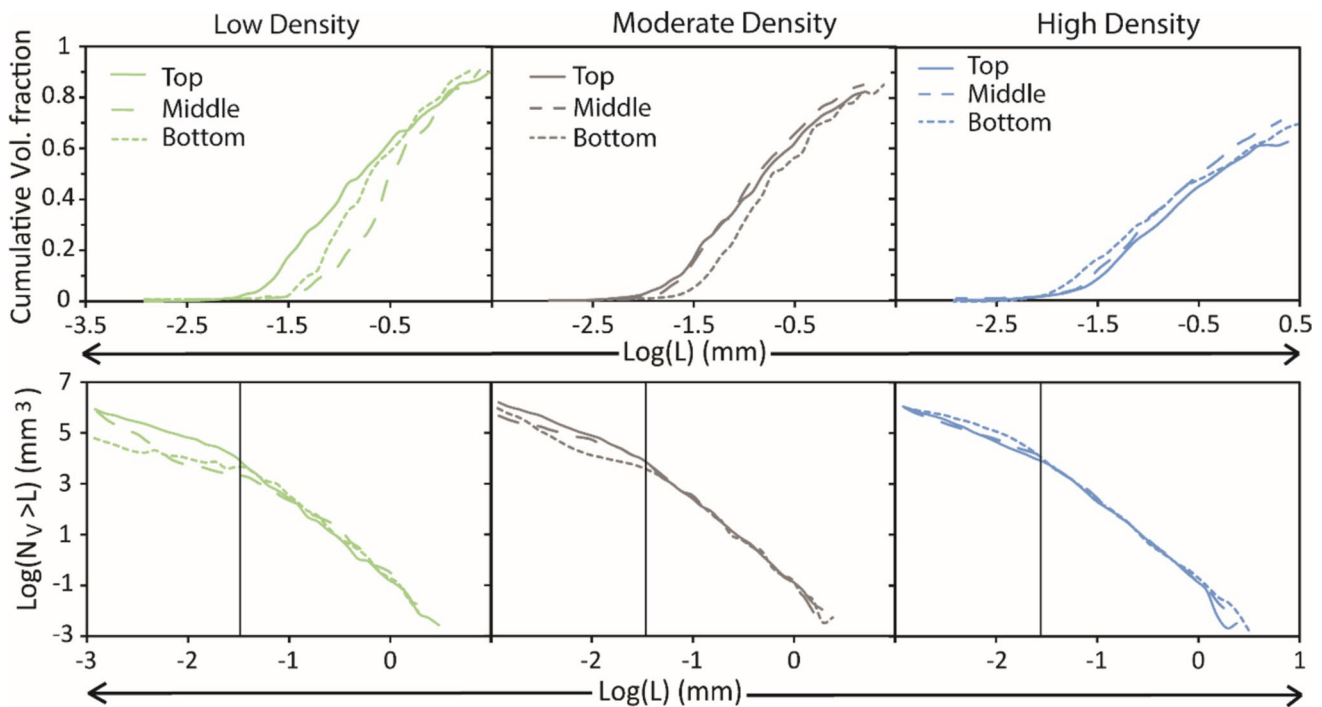
Fig. 8 Cumulative vesicle size distribution of low-, moderate-, and high-density pumice collected from bottom, middle, and top stratigraphic levels of the ~87 ka Baricha deposit. L is the equivalent vesicle diameter in mm. The multiple bulges on the cumulative volume
