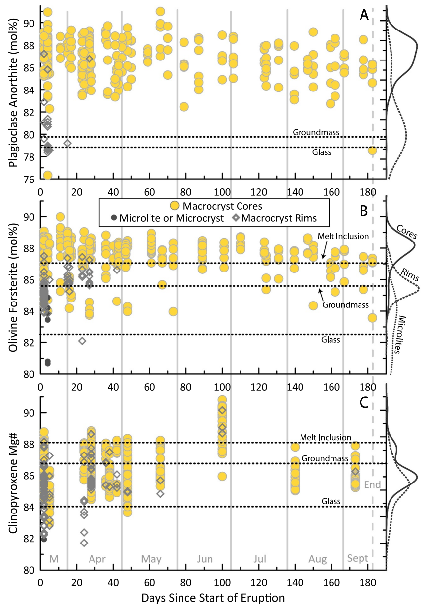
Figure 3. (a) Plagioclase anorthite content, (b) olivine forsterite content, (c) and clinopyroxene Mg# versus eruption date. The measured compositions of macrocryst cores (large yellow circles), macrocryst rims (lighter gray diamonds), and microlites and microcrysts (smaller darker gray circles) are plotted. On the right of each figure are three kernel density estimations (KDEs) of macrocryst cores (solid black line), macrocryst rims (dashed line), and microlites and microcrysts (fine dotted line). The horizontal dashed black lines represent the An, Fo, and Mg# of cpx compositions that are in equilibrium with compositions of the average lava glass, macrocryst-free matrix (groundmass), and melt inclusions. The plagioclase equilibrium line for melt inclusions is not shown because of the complexities of high-An plagioclase-melt phase equilibria (see Ustunisik et al., 2021). Plagioclase equilibrium was calculated using the model of Neave and Namur (2022). Olivine equilibrium was achieved by using a Fe-Mg Kd in the range 0.27–0.33 (Roeder & Emslie, 1970), whereas for clinopyroxene in the range 0.24–0.30 (Putirka, 2008).
