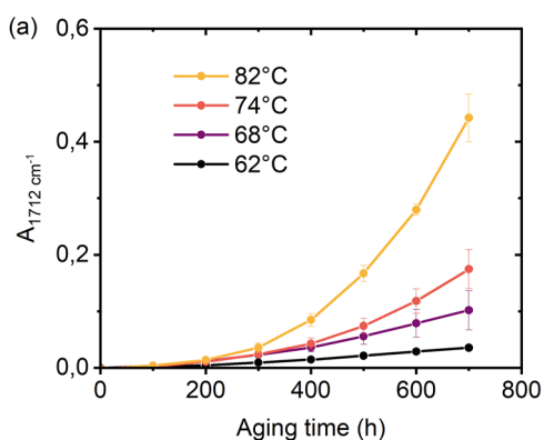
Fig. 6 | Absorbance at 1712 cm -1 (related to carboxylic acids) during TPO2 film photoaging under 305 nm LEDs at various temperatures (62, 68, 74, and 82 °C).
