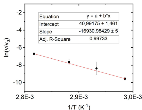
Fig. 7 | Determination of E_a for TPO2 (films irradiated under 305 nm LEDs at 20 W.m -2 ) using the Arrhenius method.
