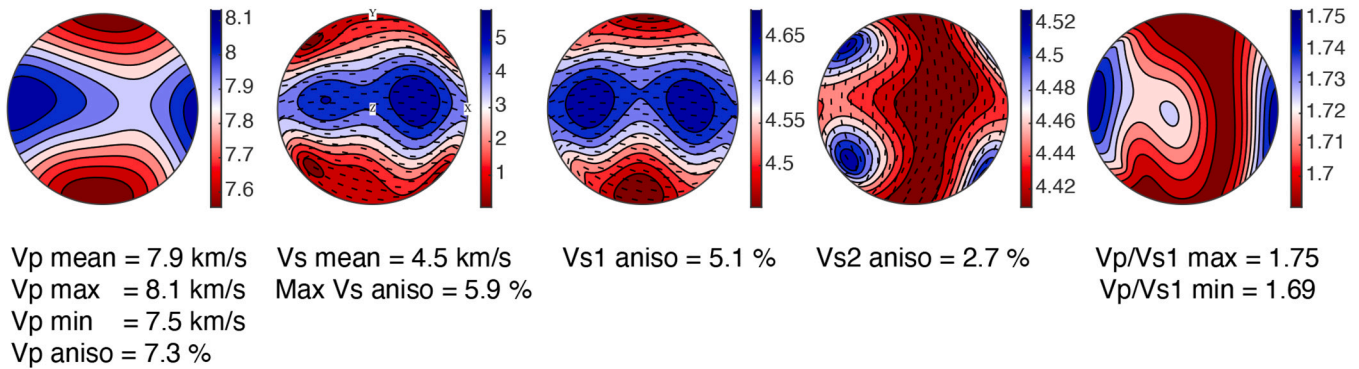
Fig. 6. Mean seismic anisotropy patterns calculated based on the 18 peridotites at 900 °C and 1.2 GPa. From left to right: P-wave velocity ( V_p ), S-wave polarization anisotropy ( AV_s ) and the orientation of fast S- wave polarization plane, S_1 wave velocities ( VS_1 ), S_2 wave velocities ( VS_2 ), and the V_p/VS_1 ratio. Lower hemisphere stereographic projection. The common deformation reference frame is indicated by the insert on the top right.
