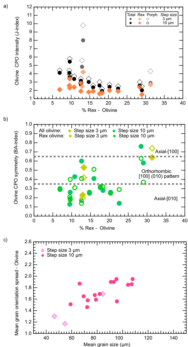
Fig. 5. (a) Texture strength (J-index) as a function of the recrystallized olivine fraction (% Rex) in Moa peridotites. A distinction is shown for EBSD maps acquired with a step size of 3 \mu\text{m} or 10 \mu\text{m} ; (b) texture symmetry (BA-index, all olivine) as a function of % Rex; (c) olivine grain orientation spread as a function of the mean grain size of olivine.
