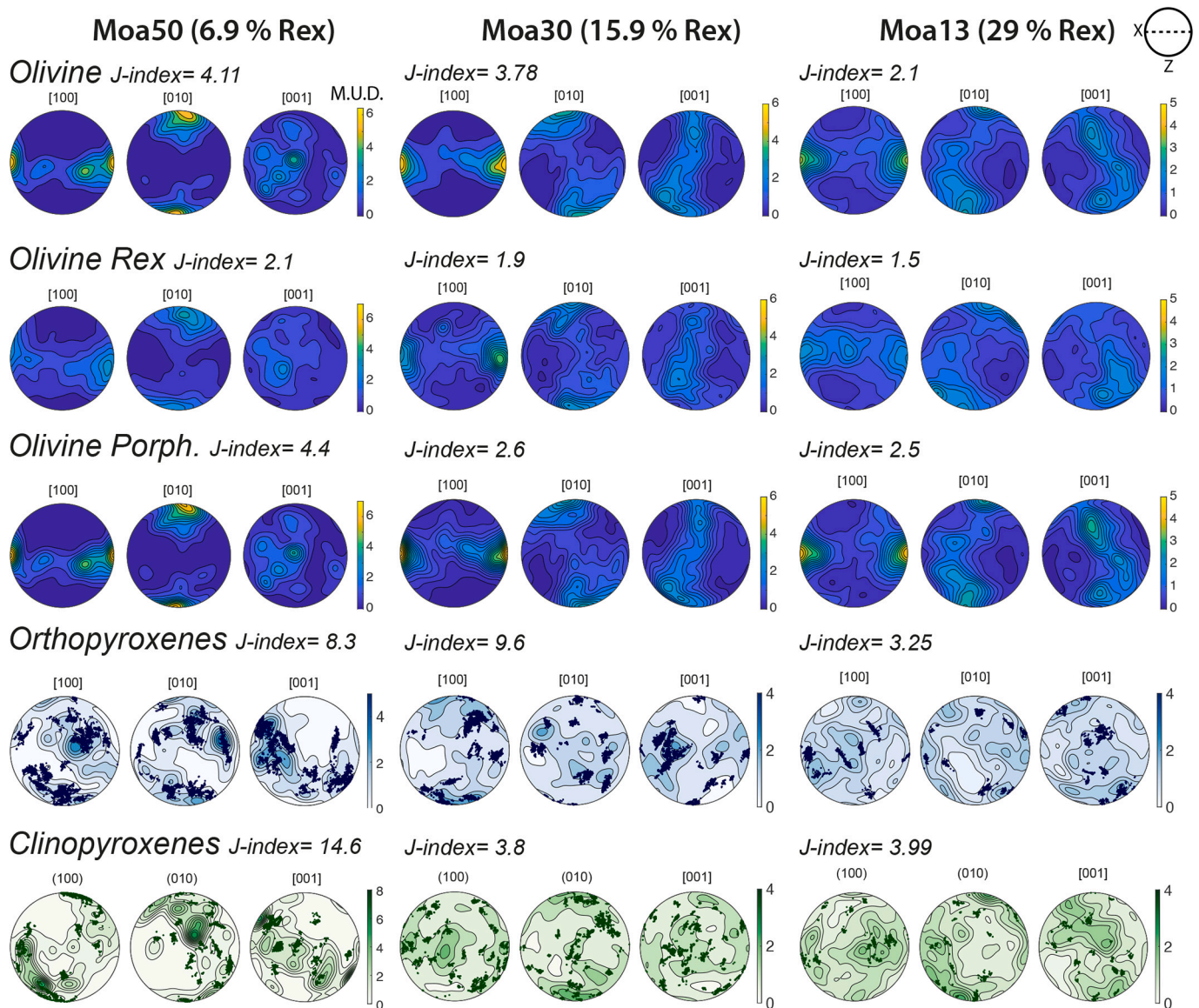
Fig. 4. Pole figures for olivine (all, % Rex = only recrystallized olivine fraction: Porph = only porphyroclastic fraction), orthopyroxene, and clinopyroxene for a selection of three representative samples with increasing amount of recrystallized olivine: Moa50 (6.9% Rex), Moa30 (15.9% Rex) and Moa13 (29% Rex). Equal-area hemisphere stereographic projections. Note that since the lineation and foliation were not well-defined in these samples, CPO are rotated to place the [100] axis maxima of olivine parallel to the x (East-West) direction (see method section for details). Contours are multiples of uniform density. Pole figures of orthopyroxene and clinopyroxene are displayed with porphyroclasts plotted as points overlaying the recrystallized fraction plotted as contours lines. The recrystallized grains of orthopyroxene are grains <250\ \mu\text{m} , and a threshold grain size of 100\ \mu\text{m} is used for clinopyroxene. NB1: if the orientation distribution of [100] of olivine is correlated with the orientation distribution of [001] of the pyroxenes, the three mineral phases are interpreted as syn-deformed . NB2: J-index = 1 is the definition of the perfectly random orientation of the crystals. See main text for details. The numbers of grains for each phase are reported in Table S2.
