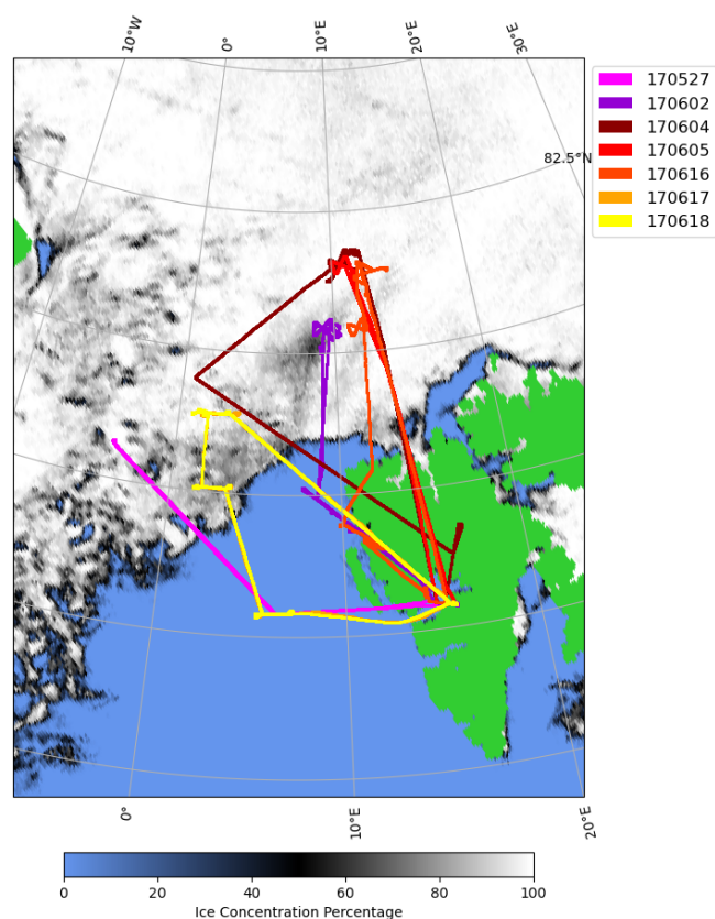
Figure 1. Flight paths for the ACLLOUD flights with Polar 6 aircraft included in the analysis overlaid on pack ice extend as of 2 June. Pack ice data are derived from measurements of the Advanced Microwave Scanning Radiometer 2 (AMSR2) at 89 GHz ( http://www.seaice.uni-bremen.de , last access: 9 November 2022; Spreen et al., 2008).
