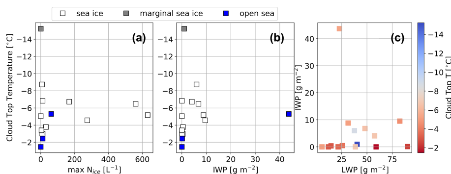
Figure 14. Maximum 10 s ice crystal number concentration ( N_{ice} ; panel a) and ice water path (IWP; panel b) as a function of cloud top temperature during ACLOUD for vertical cloud profiles over pack ice (white symbols), marginal sea ice zone (grey symbols) or the open-sea surface (blue symbols). The correlation between liquid water path (LWP) and IWP is shown in panel (c), where the symbols are colour-coded with the cloud top temperature. The list of vertical cloud profiles can be found in the Supplement.
