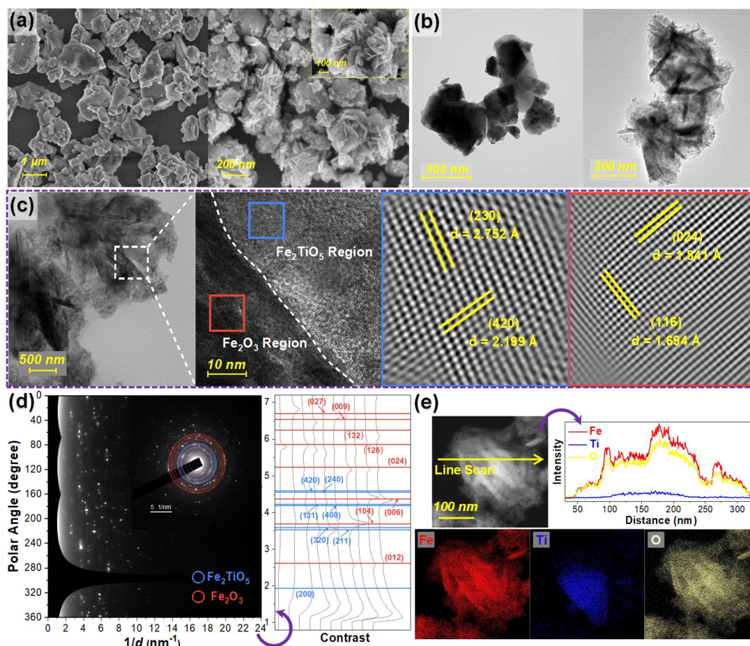
158 159 Figure 1 (a) Overall scanning electron microscope (SEM) images of raw Fe 2 TiO 5 and synthesized 160 Hem/Fe 2 TiO 5 . (b) Localized TEM images of Fe 2 TiO 5 and Hem/Fe 2 TiO 5 . (c) High-resolution TEM 161 and filtered inverse fast Fourier transform (IFFT) images with lattice fringe markings of 162 Hem/Fe 2 TiO 5 . (d) SAED patterns with a polar coordinate expansion of localized Hem/Fe 2 TiO 5 . (e) 163 EDS mapping and Line scan images of typical Hem/Fe 2 TiO 5 composite region.
