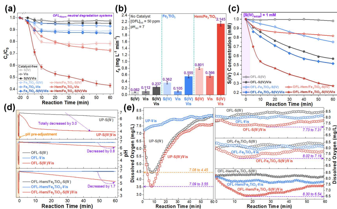
283 Figure 3 (a) Degradation of OFL in various catalyst-S(IV)/Vis systems. (b) Corresponding initial 284 reaction rates within different systems. (c) Changes of S(IV) concentration under different catalytic 285 conditions. Continuous monitoring curves for pH (d) and DO (e) in various control experiments. 286 Conditions: [OFL] = 50 ppm, [Catalyst] = 0.5 g/L, [S(IV)] = 1 mM, pH = 7, under Vis-irradiation.
