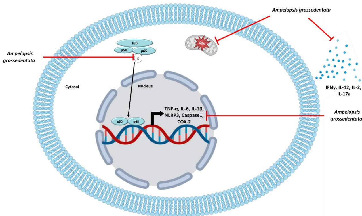
Figure 6. Anti-inflammatory mechanisms of APG extract. IL-2: interleukin-2; IL-6: interleukin-6; IL-12: interleukin-12; IL-17a: interleukin-17a; IL-1 \beta : interleukin-1 \beta , IFN \gamma : interferon gamma; TNF- \alpha : tumor necrosis factor; COX-2: cyclooxygenase-2; NLRP3: NLR Family Pyrin Domain-Containing 3; ROS: reactive oxygen species.
