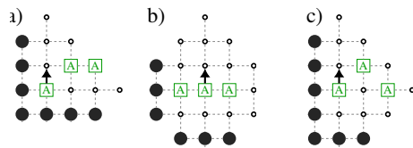
Fig. 24: Rules to turn after exploring the first row.
