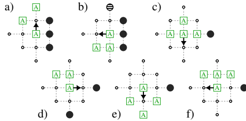
Fig. 8: Rules to move the sentinel to the next row to be explored.
