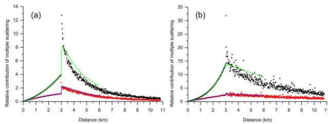
Figure 7. Monte Carlo simulations of multiple-scattering, R_{MSto1} (black points), and double-scattering, R_{2to1} (red points), relative contributions to lidar signals. (a) Water cloud. (b) Jet-stream cirrus. Eloranta model simulations are shown by the green (MS) and the blue (DS) curves.
