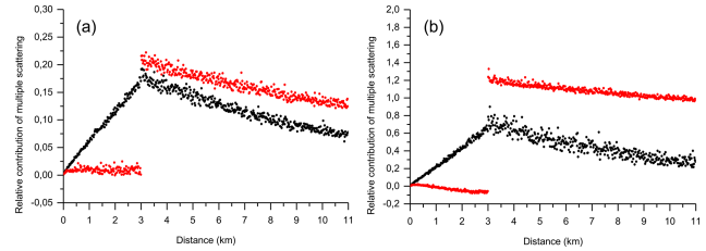
Figure 9. Monte Carlo simulations of multiple-scattering effects (jet-stream cirrus). Black points are the relative contributions, R_{\text{MSto1}} , to lidar signals from a homogeneous plane-parallel cloud; red points are the relative contributions, R_{\text{NUBFto1}} , of the MS and the NUBF to lidar signals from a 3D cloud. The extinction coefficients are (a) 0.06 \text{ km}^{-1} and (b) 0.2 \text{ km}^{-1} .
