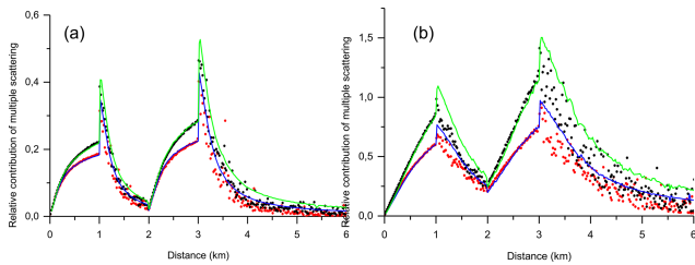
Figure 5. Monte Carlo simulations of multiple-scattering, R_{MSto1} (black points), and double-scattering, R_{2to1} (red points), relative contributions to lidar signals. (a) Water cloud. (b) Jet-stream cirrus. Eloranta model simulations are shown by the green (MS) and the blue (DS) curves.
