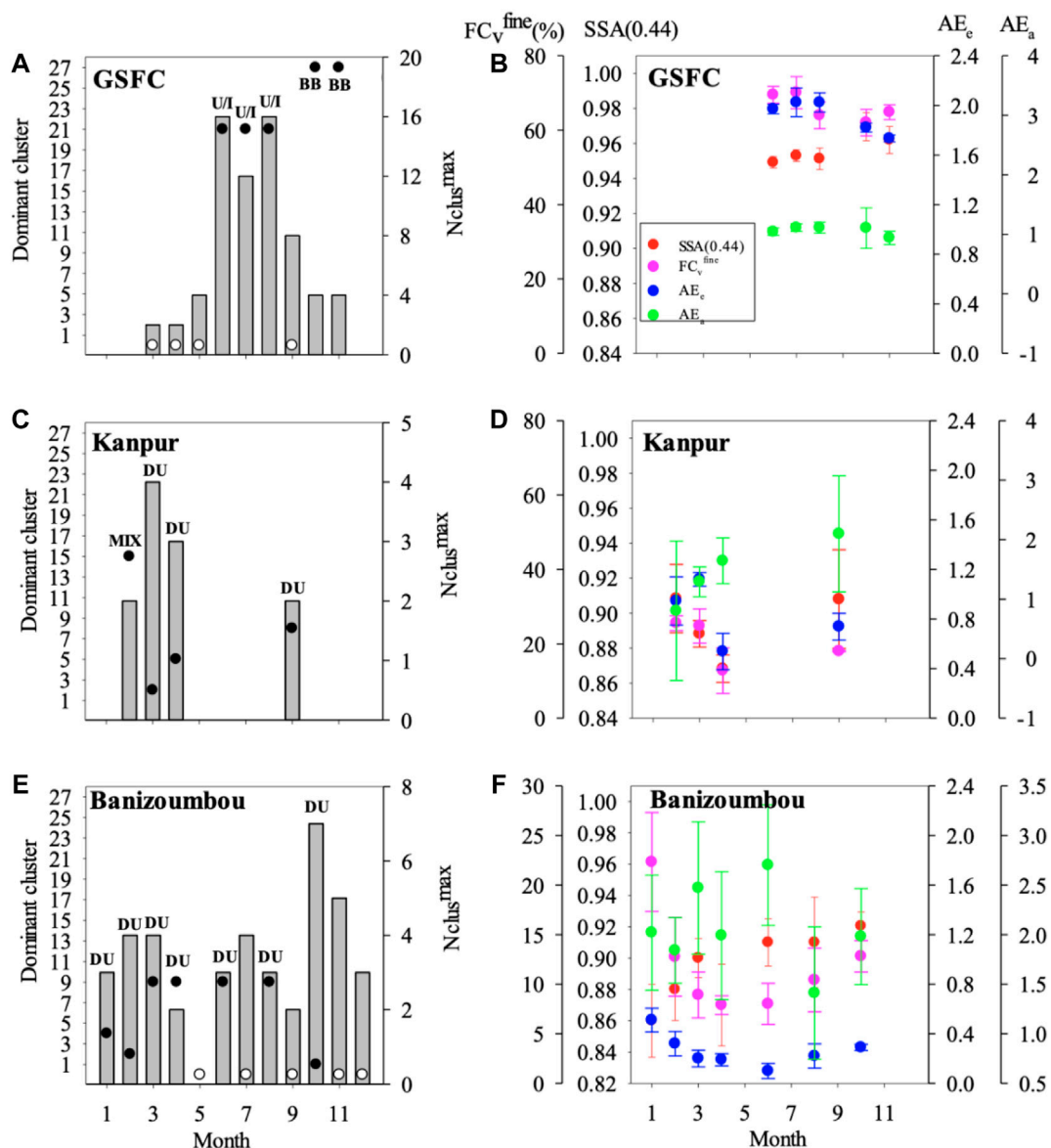
FIGURE 7 | Site-specific monthly variability of PAM-derived aerosols. GSFC (A, B), Kanpur (C, D), Banizoumbou (E, F), dominant aerosol sub-type ids (left panels, solid circles), types (bold legend) and their mean properties (right panels), co-dominance of clusters (left panels, empty circles), N_{clus}^{max} is the number of records for the dominant cluster.
