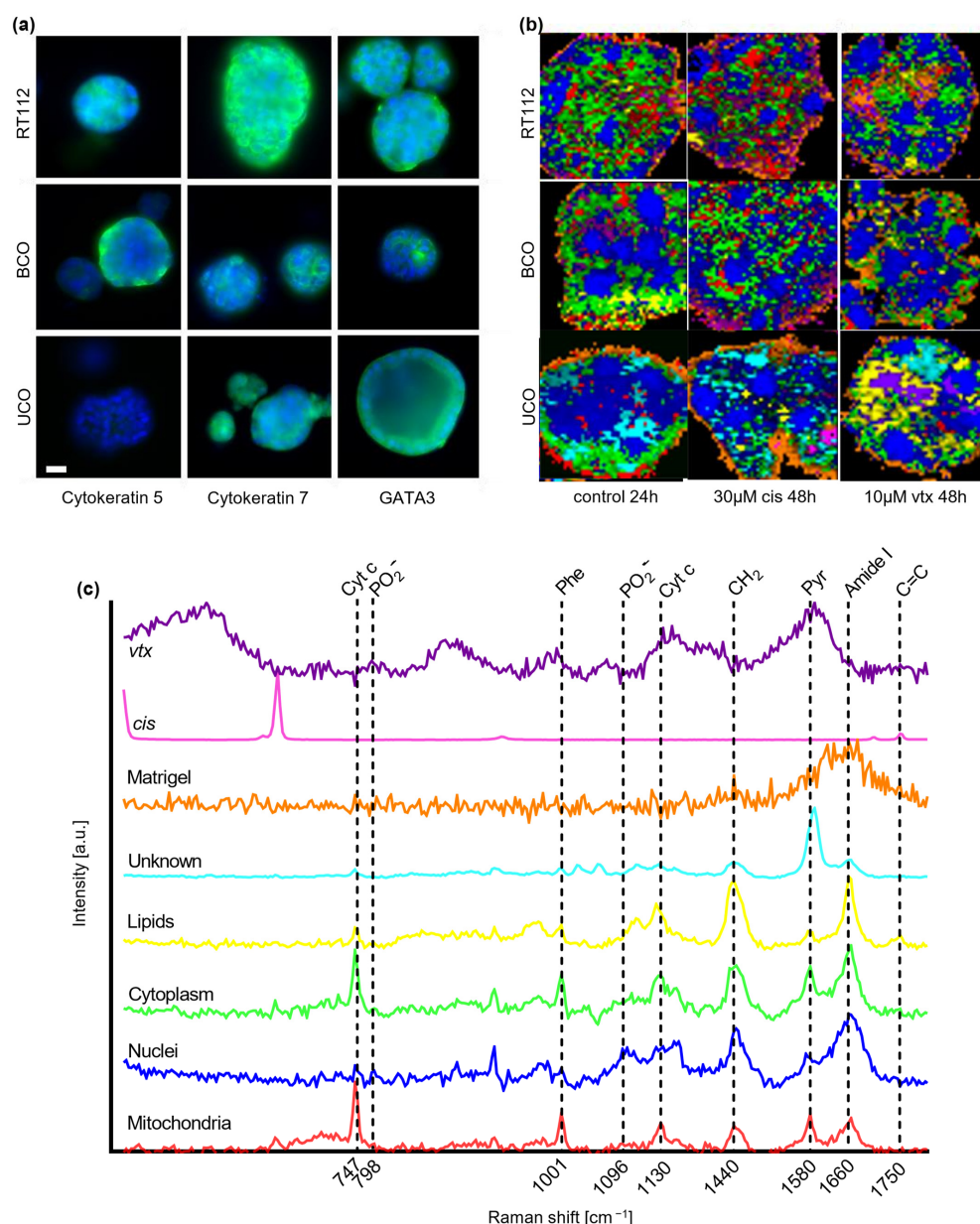
Figure 1. Immunofluorescence (IF) and Raman microspectroscopy (RMS) of different bladder cancer organoid models. (a) IF images of untreated RT112, BCO and UCO organoids stained for cytokeratin 5, cytokeratin 7 or GATA3 (green) and DAPI (blue). Scale bar: 25 μm. (b) True component analysis (TCA) images of RT112, BCO and UCO organoids. Displayed is one representative scan of untreated and treated organoids (30 μM cisplatin ( cis ) or 10 μM venetoclax ( vtx )) for each organoid model. Scale bar: 20 μm. (c) Relevant TCA spectra for the identified cellular components.
