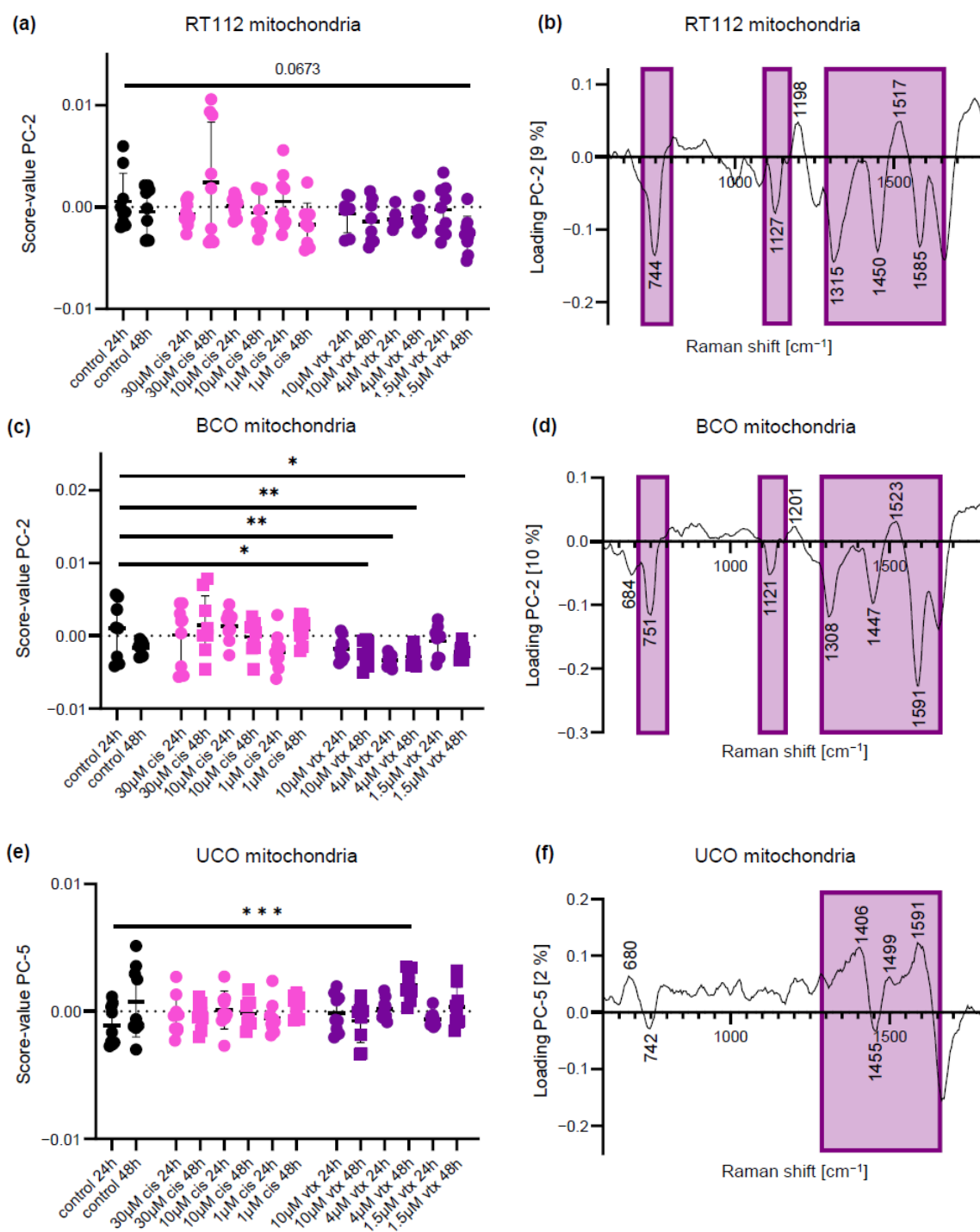
Figure 3. PCA of mitochondria-derived Raman spectra reveals similar spectral for all organoid models after vtx (purple) treatment. (a) Score value analysis of organoids from the cell line RT112 shows tendencies of separation after vtx treatment. (b) Corresponding loading plot. (c) Score value analysis of patient-derived BCOs show statistically significant differences after vtx . (d) Corresponding loading plot. (e) Score value analysis of patient-derived UCOs reveals statistically significant differences between controls and vtx treatment. (f) Corresponding loading plot. Black: controls; pink: cis treatment; purple: vtx treatment; circles: 24 h; square: 48 h; Statistical analysis: One-way ANOVA, n = 9 , * p < 0.05 , ** p < 0.01 , *** p < 0.001 .
