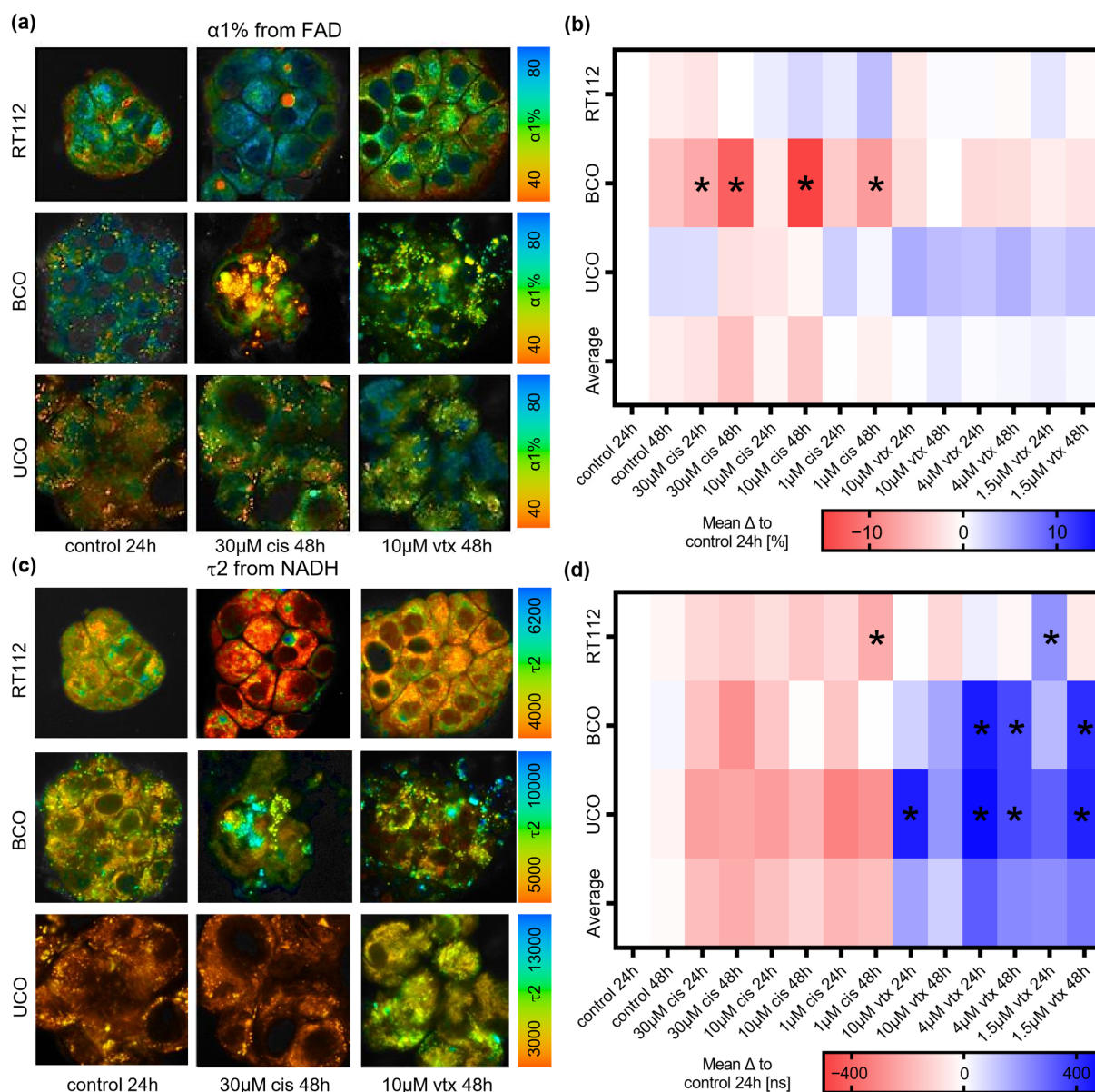
Figure 6. FLIM of bladder cancer organoids. (a) Representative FAD \alpha 1\% images of control RT112, BCO and UCO organoids and 48 h after 30 \mu\text{M} cis or 10 \mu\text{M} vtx treatment. Scale bar: 25 \mu\text{m} . (b) Heatmap of mean differences of NADH \alpha 1\% to the 24 h control. (c) Representative NADH \tau 2 images of control RT112, BCO and UCO organoids and 48 h after 30 \mu\text{M} cis and 10 \mu\text{M} vtx treatment. Scale bar: 25 \mu\text{m} . (d) Heatmap of mean differences of NADH \tau 2 to the 24 h control. One-way ANOVA, n = 15 , * p < 0.05 .
