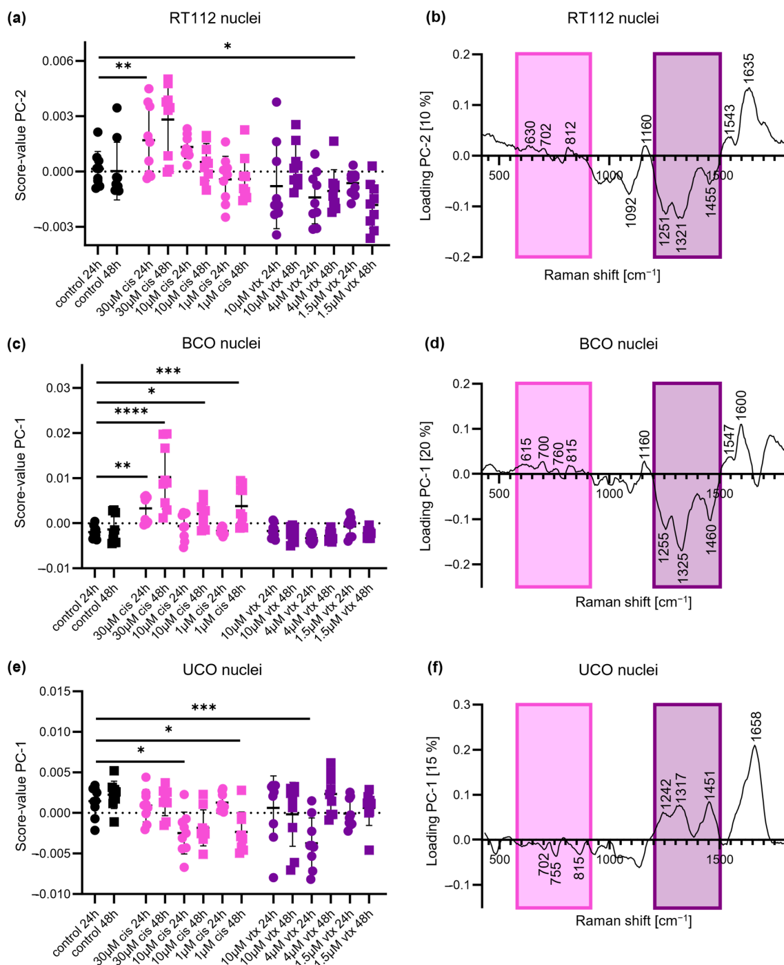
Figure 2. PCA of nuclei-derived Raman spectra reveals similar spectral changes for all organoid models after cis (pink) and vtx (purple) treatments. (a) Score value analysis of the cell line RT112 shows statistically significant differences after cis and vtx treatment. (b) Corresponding loading plot. (c) Score value analysis of patient-derived BCOs shows statistically significant differences after cis treatment and tendencies of separation after vtx treatment. (d) Corresponding loading plot. (e) Score value analysis of patient-derived UCOs reveals statistically significant differences between controls and cis and vtx treatment. (f) Corresponding loading plot. Black: controls; pink: cis treatment; purple: vtx treatment; circles: 24 h; square: 48 h; Statistical analysis: One-way ANOVA, n = 9 , * p < 0.05 , ** p < 0.01 , *** p < 0.001 , **** p < 0.0001 .
