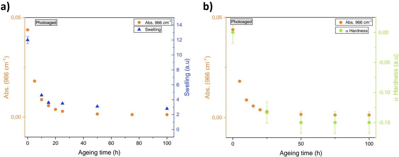
Figure 17. (a): Absorbance at 966\text{ cm}^{-1} (●) and swelling (▲) versus photooxidation time, (b): Absorbance at 966\text{ cm}^{-1} (●) and shore A hardness conversion rate (◆) versus photooxidation time
