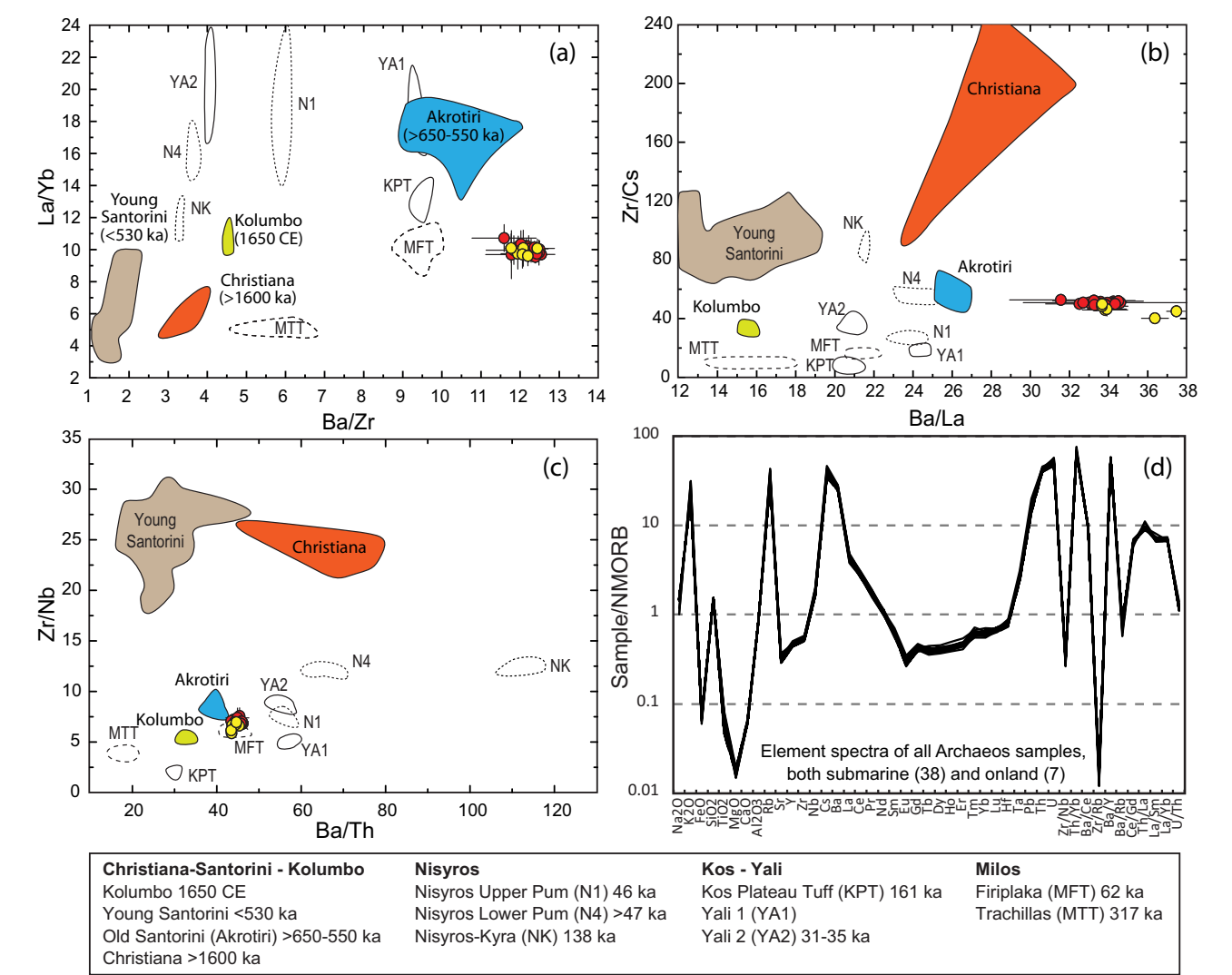
Fig. 4 Chemical compositions of glasses from the Archaeos Tuff. a–c Incompatible trace element ratio plots showing the compositional similarity of onland (yellow dots) and offshore (red dots) samples of the Archaeos Tuff to those of the Early Centres of Akrotiri (>650–550 ka), and the differences with other volcanic centres of the South Aegean Volcanic Arc and the younger tuffs of Santorini (<530 ka). Data points denote means and standard deviations. All the analyses are glasses 19 , apart from Christiania, which are whole-rock lavas with >60 % SiO 2 . d Glass element spectra normalized to N-MORB for 38 offshore samples (at seven drill sites shown in red in Fig. 1) and 7 onshore samples (yellow locations in Fig. 1) of the Archaeos Tuff, showing the essentially identical compositions.
