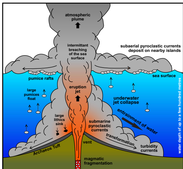
Fig. 6 Schematic depicting eruption and emplacement of the Archaeos Tuff 520 \pm 10 \text{ ky} ago. The eruption took place from one or more shallow submarine vents of the ancient Akrotiri Volcano 17 in the Santorini-Christiania area. The vent was situated in water shallow enough for magma fragmentation to occur mainly by the exsolution and expansion of magmatic gases 1 . Orange colours in the jet denote higher temperatures. As the gas-particle mixture of the eruption jet rose through the water column, it ingested water and partially collapsed to form submarine pyroclastic currents 2-4 . These currents in turn entrained more water and transformed into turbidity currents and slurries that spread out across the sea floor 11-13 laying down a volcanoclastic megaturbidite up to 150 m thick. Breaching of the sea surface by the eruption column also generated subaerial pyroclastic currents that travelled across the sea surface and pumice rafts 56-59 , and deposited thin veneers of ignimbrite on the islands (not shown) of Christiani, early Santorini, and Anafi. The cartoon is exaggerated vertically, being several km across and about a km high.
