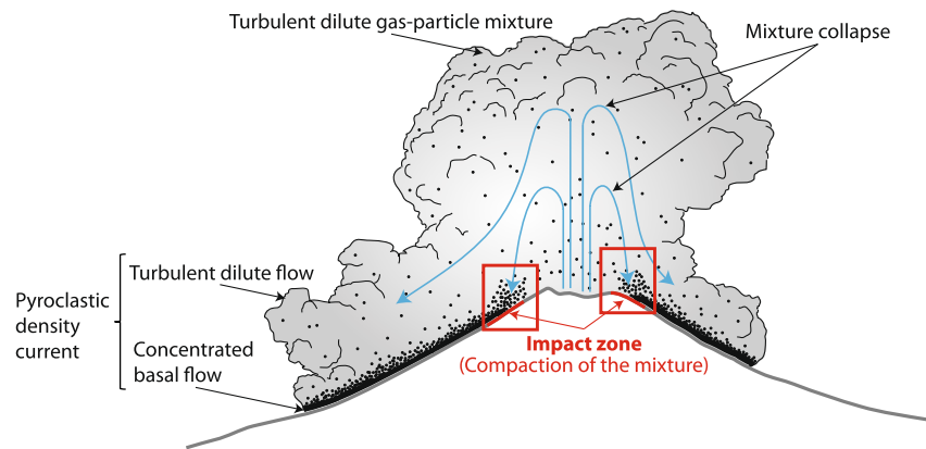
Figure 1. Sketch of a pyroclastic fountain. A gas-particle mixture emitted from the vent experiences gravitational collapse. Pyroclastic density currents emerge from impact zones and consist of a concentrated basal part topped by a dilute suspension. The gas phase corresponds to gray shades and particles are represented by black dots.
