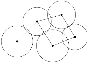
FIGURE 1. A triangle-free intersection graph of disks in the plane, and the associated planar graph embedding.
