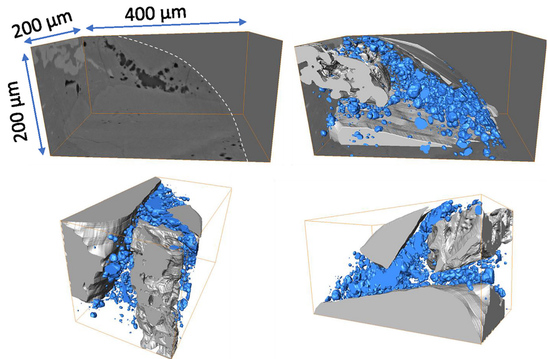
Figure 5. Synchrotron-based X-ray microtomography at a voxel size of 360 nm revealing the presence of a fourth vesicle type, forming vesicle trains along crystal boundaries, with vesicles and crystals represented in blue and gray in 3D renderings, respectively.
