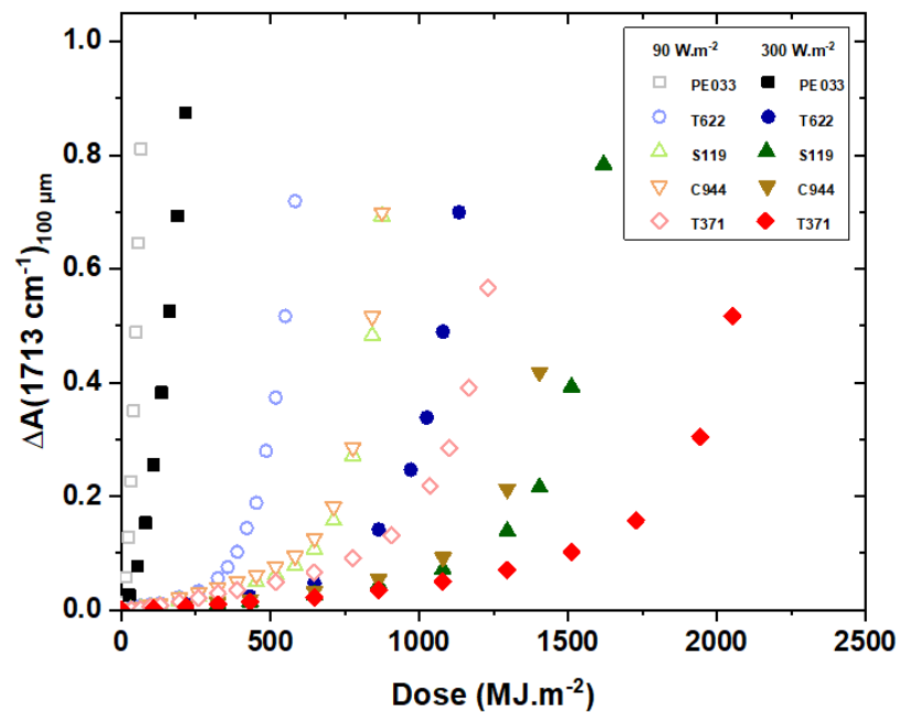
Figure 8. Carbonyl absorbance \Delta A(1713 \text{ cm}^{-1}) vs. dose (in \text{MJ.m}^{-2} ) at 90 and 300 \text{W.m}^{-2} for formulations presented in Table 2 and Figure 3 ( T = 60 \text{ }^\circ\text{C} and film thickness = 100 microns)
