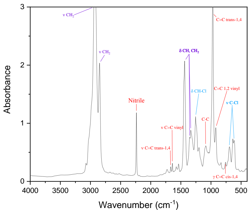
Figure 1. FTIR spectrum of NBR/PVC blend film (e= 115 μm) before ageing
