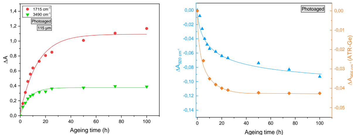
Figure 6. Absorbance variation at (a): 1715 cm -1 (●) and 3490 cm -1 (▼) and (b): 920 cm -1 (▲) and 966 cm -1 (◆) during NBR/PVC film photooxidation
