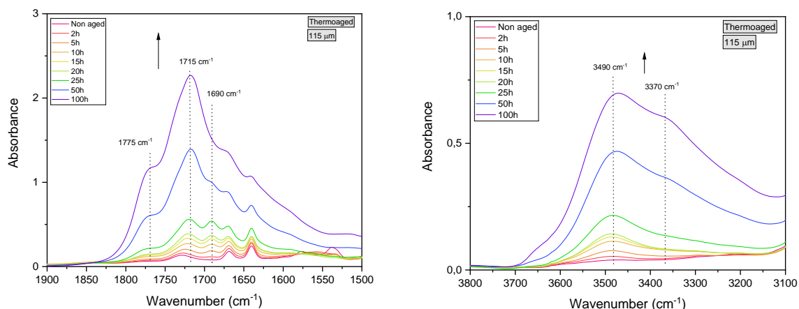
Figure 7. FTIR spectra in (a): the carbonyl region (1900-1500 cm -1 ) and (b): the hydroxyl region (3800-3100 cm -1 ) of the NBR/PVC film during thermooxidation
