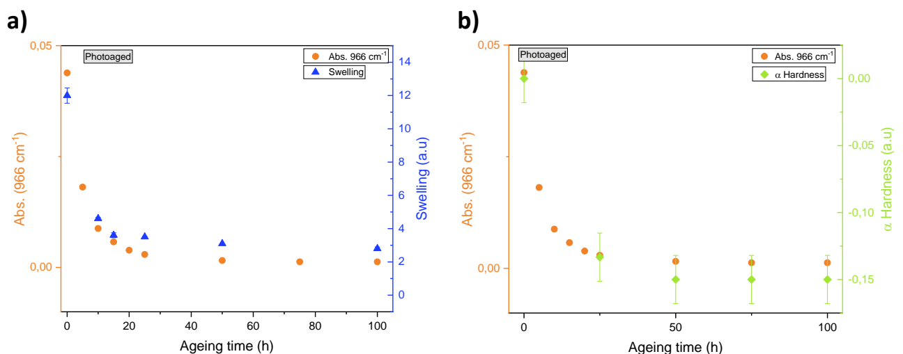
Figure 17. (a): Absorbance at 966 \text{ cm}^{-1} (●) and swelling (▲) versus photooxidation time, (b): Absorbance at 966 \text{ cm}^{-1} (●) and shore A hardness conversion rate (◆) versus photooxidation time
