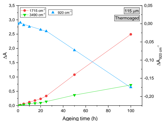
Figure 8. Absorbance variation at 920 \text{cm}^{-1} (▲), 1715 \text{cm}^{-1} (●) and 3490 \text{cm}^{-1} (▼) during NBR/PVC film thermooxidation
