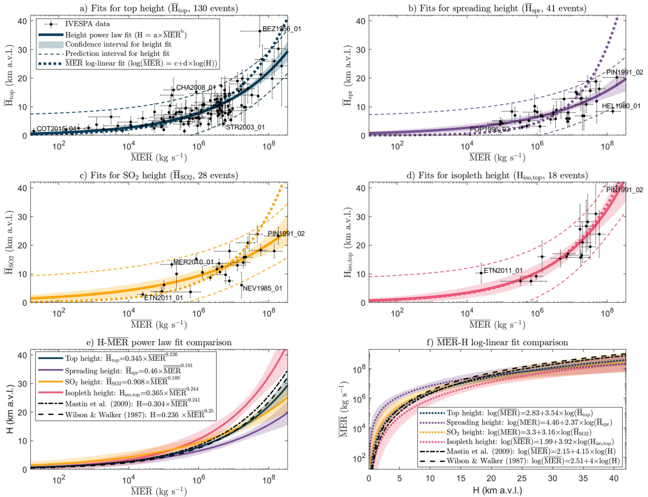
Figure 1. \bar{H}_{\text{top}} (a), \bar{H}_{\text{spr}} (b), \bar{H}_{\text{SO}_2} (c) and H_{\text{iso,top}} (d) as a function of \overline{\text{MER}} . Panels (e) (power law fit, \overline{\text{MER}} as independent variable) and (f) (log linear fit, height as independent variable) compare the new empirical relationships for the four heights considered, along with relationships from Mastin et al. (2009) and Wilson and Walker (1987). Select events on panels (a)–(d) are labeled using their Independent Volcanic Eruption Source Parameter Archive (IVESPA) identifiers (see Table S1 for full details), for example, PIN1991_02 is phase 2 of the 1991 eruption of Mount Pinatubo.
