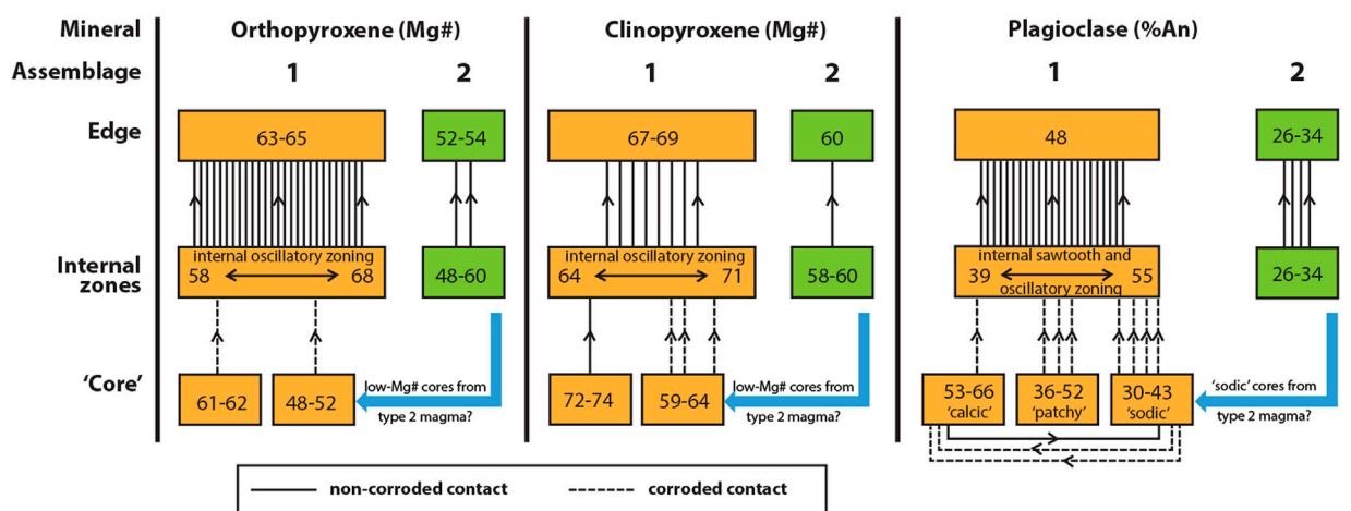
FIGURE 4 Summary of the zoning patterns in opx, cpx and plagioclase of the PKP, from core to crystal edge. The numbers are Mg# Numbers (for opx and cpx) or An contents (for plagioclase). Arrows show the inclusion of one compositional group within another, associated with a conformable (solid arrow) or corroded (dashed arrow) contact. Orange boxes are compositions within type 1 crystals, and green boxes are those within type 2 crystals. The blue arrows show evidence for the inclusion of type 2 crystals as cores within some type 1 crystals.
