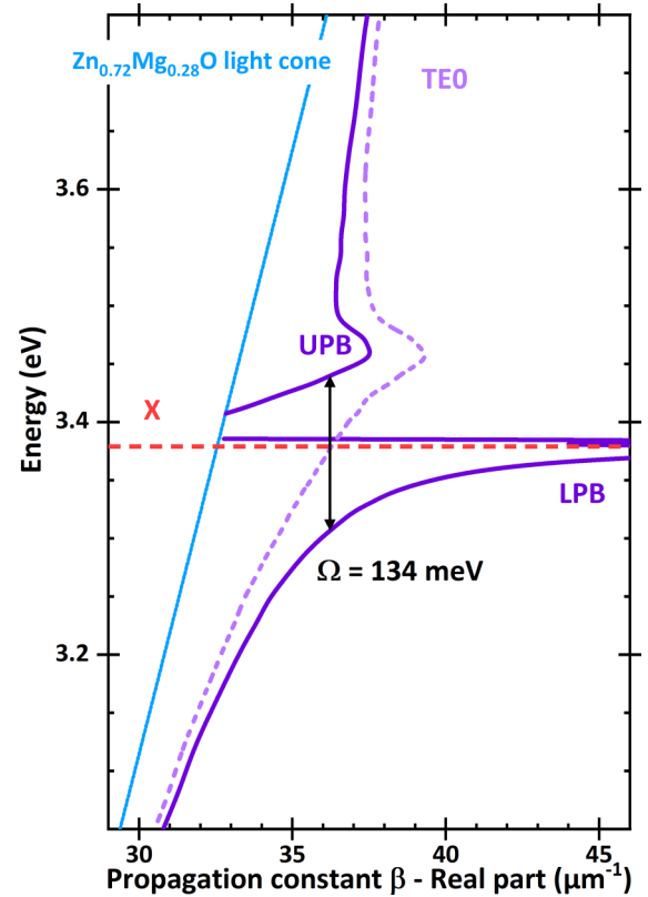
FIG. 2. Numerical calculation of the guided polariton dispersion in purple showing a Rabi splitting of 134 meV between the lower and upper branches. The TE 0 photonic mode (light purple dashed line) is obtained using only the background permittivity of ZnO without excitonic contributions. The \text{Zn}_{0.72}\text{Mg}_{0.28}\text{O} light cone (light blue) corresponds to a linear dispersion with a constant refractive index of 1.9. The red dotted line indicates the mean energy of the excitonic transitions.
