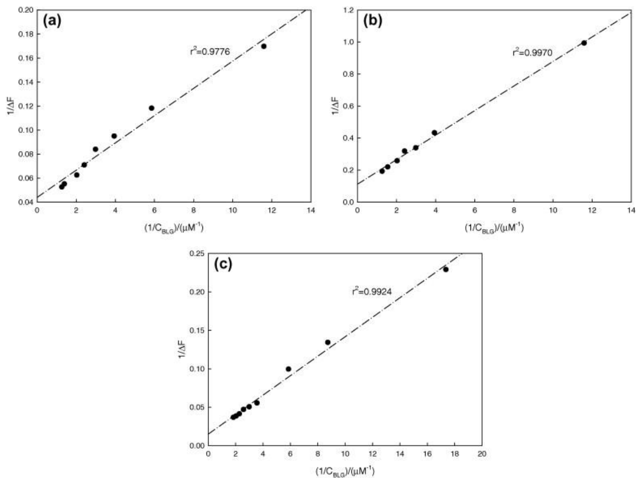
FIGURE 7. The linear plots of 1/\Delta F as a function of 1/C_{\text{BLG}} based on equation (7) and in the presence of various C_{16}\text{TAB} concentrations; (a) 50 \mu\text{M} , (b) 200 \mu\text{M} , and (c) 500 \mu\text{M} .
