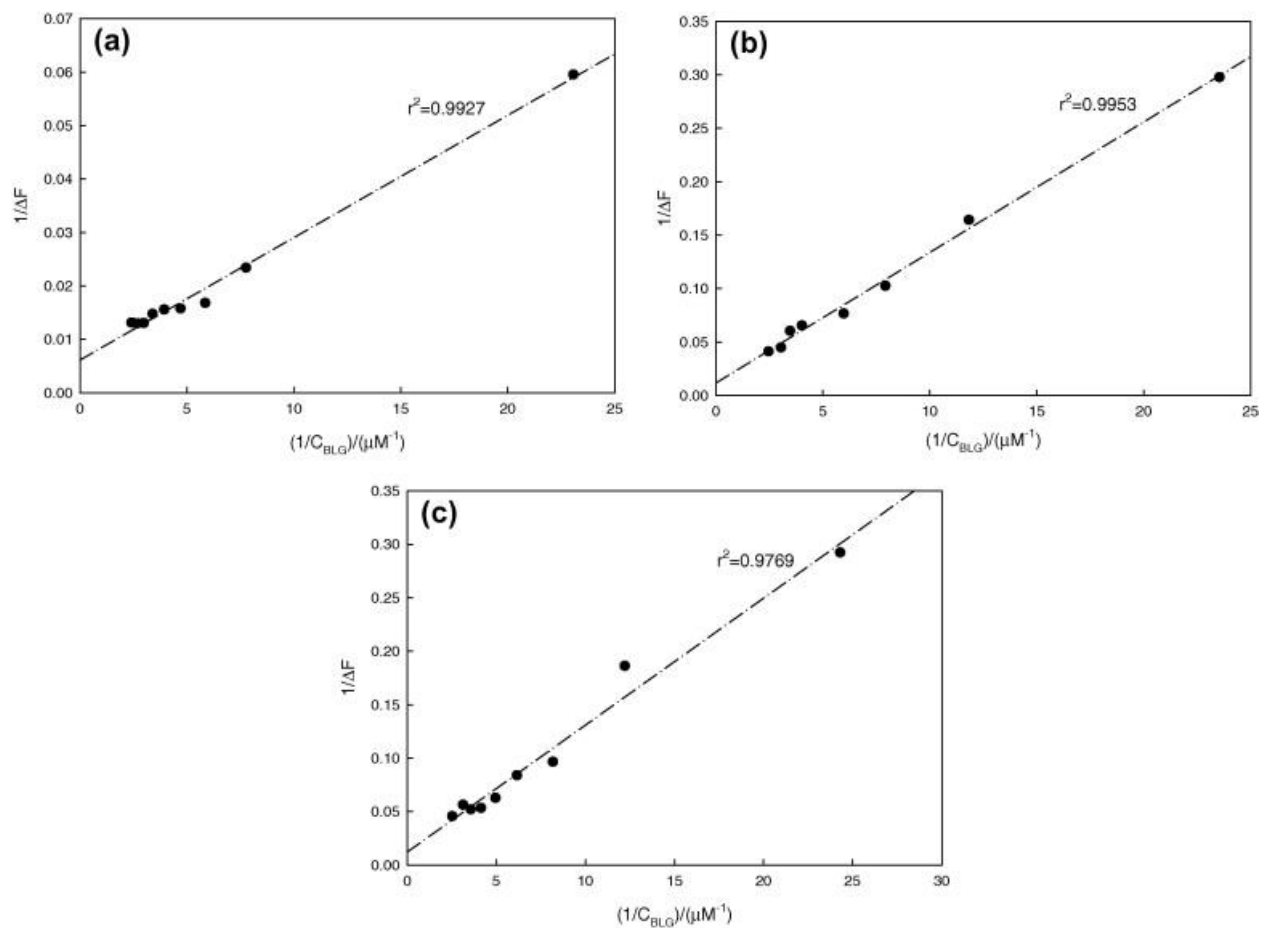
FIGURE 6. The linear plots of 1/\Delta F as a function of 1/C_{BLG} based on equation (7) and in the presence of various C_{14TAB} concentrations; (a) 100 \mu M , (b) 300 \mu M , and (c) 600 \mu M .
