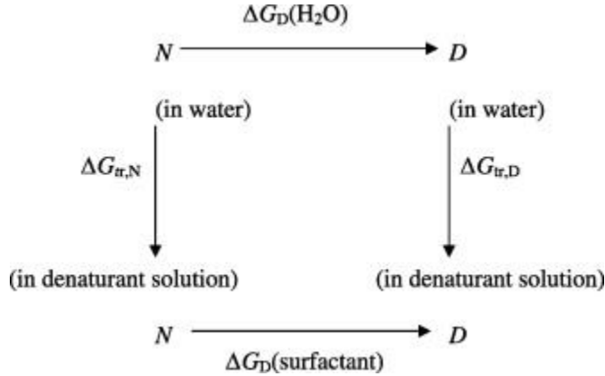
SCHEME 1. Unfolding BLG in an isothermal chemical denaturation process.
