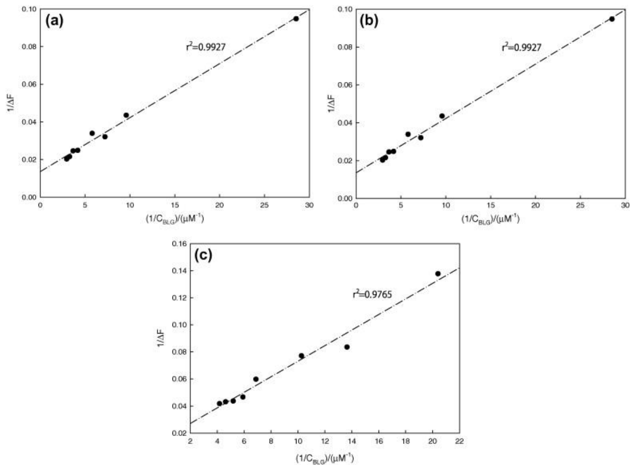
FIGURE 5. The linear plots of 1/\Delta F as a function of 1/C_{BLG} based on equation (7) and in the presence of various C_{12TAB} concentrations; (a) 500 \mu M , (b) 2.0 mM, and (c) 2.8 mM.
