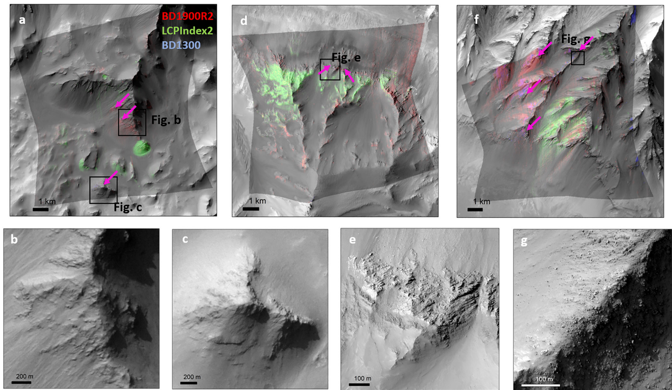
Figure 3. a- CRISM FRT00008112 color composite of image summary parameters R = BD1900R2, G = LCPINDEX2 and B = BD1300 are projected in transparency over CTX image F20_043546_1695_XN_10S048W of the northern walls of Capri Chasma. This color composite highlights LCP-rich bedrock outcrops in green, clay-bearing outcrops in red and mixed clays and feldspars in magenta (see arrows as well). (b, c) Close-ups on feldspar-bearing outcrops on the same CTX image. (d) CRISM FRT00009226 RGB composite of the same summary parameters are projected in transparency over CTX image P15_006717_1643_XI_15S054W. e-Close-up on feldspar-bearing outcrops on corresponding High Resolution Imaging Science Experiment (HiRISE) image PSP_006717_1655 (f) CRISM FRT0000B8E2 RGB composite of the same summary parameters are projected in transparency over CTX image P15_006717_1643_XI_15S054W. (g) Close-up of feldspar-bearing outcrops on corresponding HiRISE image PSP_009222_1660.
