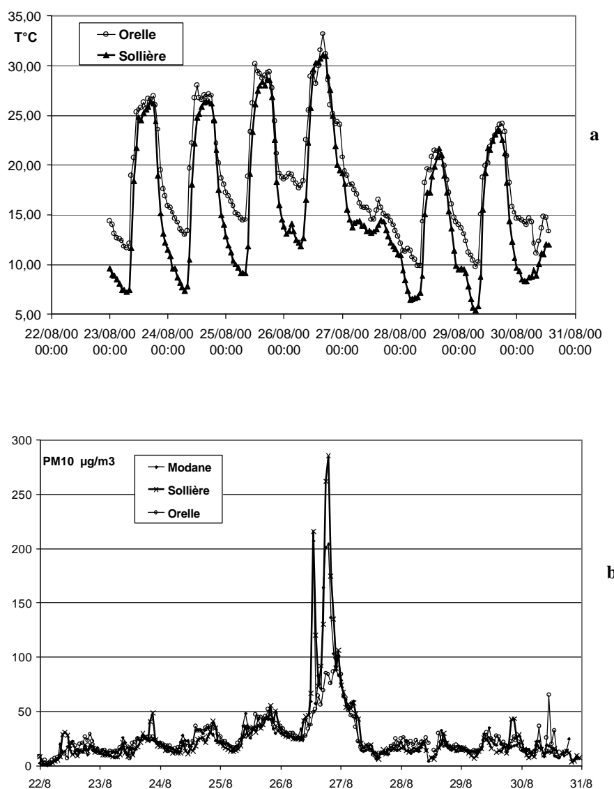
FIGURE 2a - Hourly average temperatures(°C)
