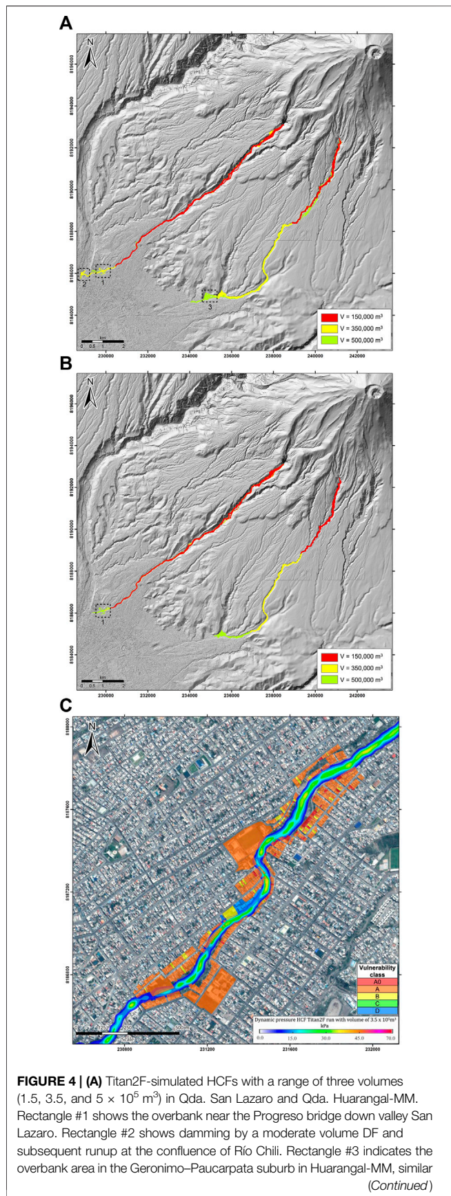
FIGURE 4 | to the actual overbank area inundated in 2011. (B) Titan2F-simulated DFs with a range of three volumes ( 2.5 , 3.5 , and 5 \times 10^5 \text{ m}^3 ) in Qda. San Lazaro and Qda. Huarangal-MM. (C) Distribution of HCF dynamic pressure (using Titan2F) in the middle reach of Qda. San Lazaro with a volume of 3.5 \times 10^5 \text{ m}^3 .
