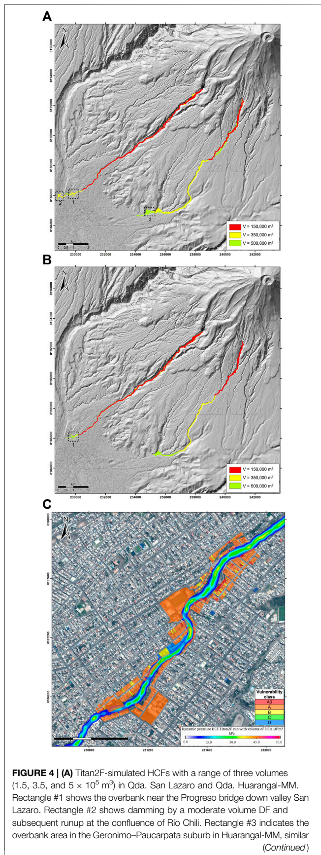
FIGURE 4 | to the actual overbank area inundated in 2011. (B) Titan2F-simulated DFs with a range of three volumes ( 2.5 , 3.5 , and 5 \times 10^5 \text{ m}^3 ) in Qda. San Lazaro and Qda. Huarangal-MM. (C) Distribution of HCF dynamic pressure (using Titan2F) in the middle reach of Qda. San Lazaro with a volume of 3.5 \times 10^5 \text{ m}^3 .
