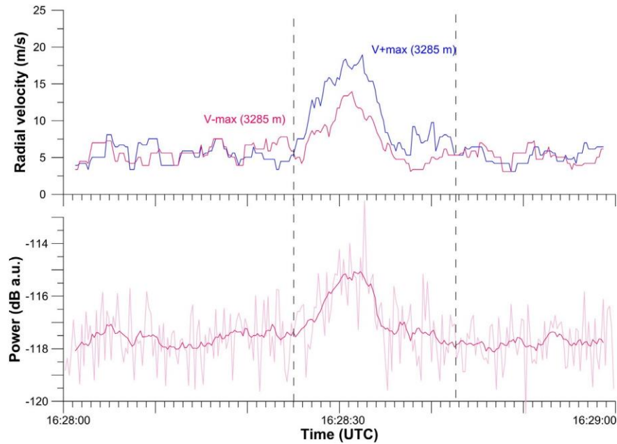
Fig. 5. VOLDORAD 2B records of the 8 April 2010 ash plume from the new pit crater on eastern flank of Etna's SE Crater. The radar time series show echo power and maximum radial velocities measured in the 3285 m range gate (see Fig. 1c).
