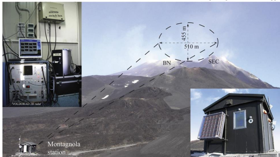
Fig. 2. Perspective view of the VOLDORAD 2B radar system (left inset) in the La Montagnola shelter (right inset), about 3.1 km south of the SE Crater (photo F. Donnadiu, July 2009).
