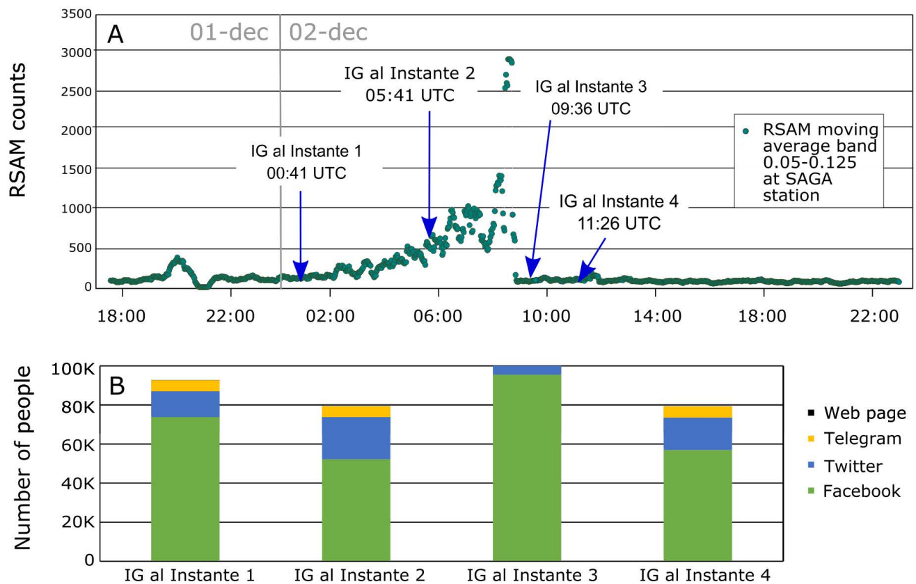
Figure 13: [A] RSAM moving average combined with the communication of eruptive process showing the time of publication for IGallInstante reports and their reach out in our social media channels, [B] Bar chart of the number of people reached by the IGallInstante publications.
