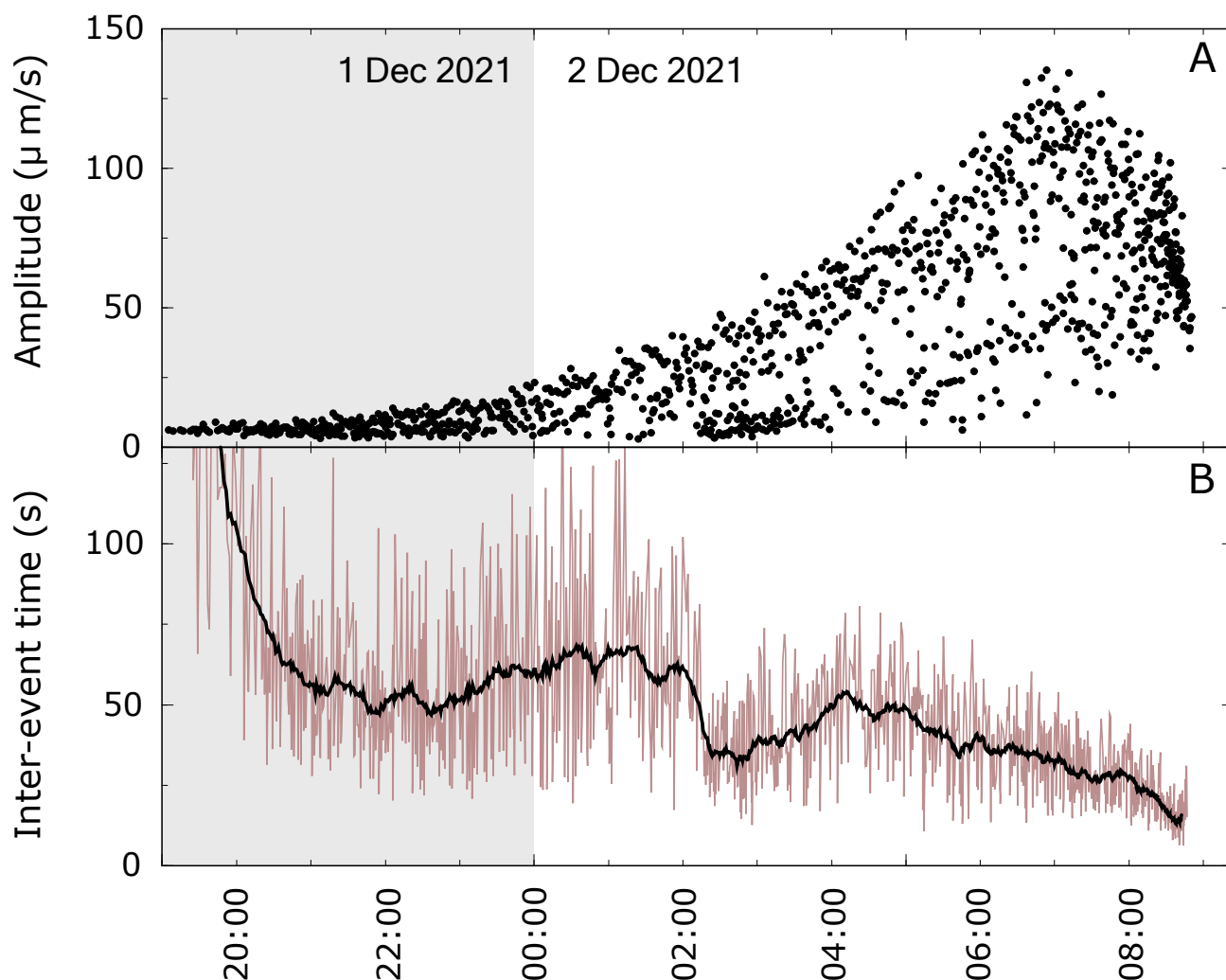
Figure 11: Seismic characteristics of the drumbeat sequence, [A] Peak to peak amplitude of the events detected by matched filtering. [B] Inter-event time for events recorded during the sequence before merging into tremor. Individual measurements are shown in the background (brown) with the black curve in foreground presenting an averaging over 30-point moving windows.
