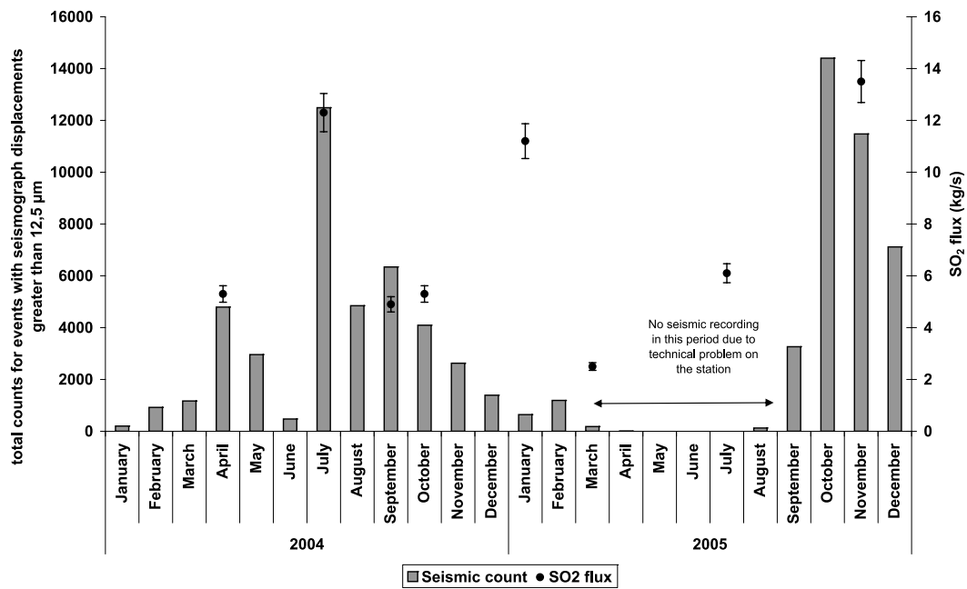
Figure 3. Correlation between seismic counts and SO 2 fluxes; volcanic events with seismograph displacements greater than 12.5 μm were recorded and plotted here from the period between January 2004 and December 2005. The SO 2 flux for each measurement period (P) is represented by circles.
