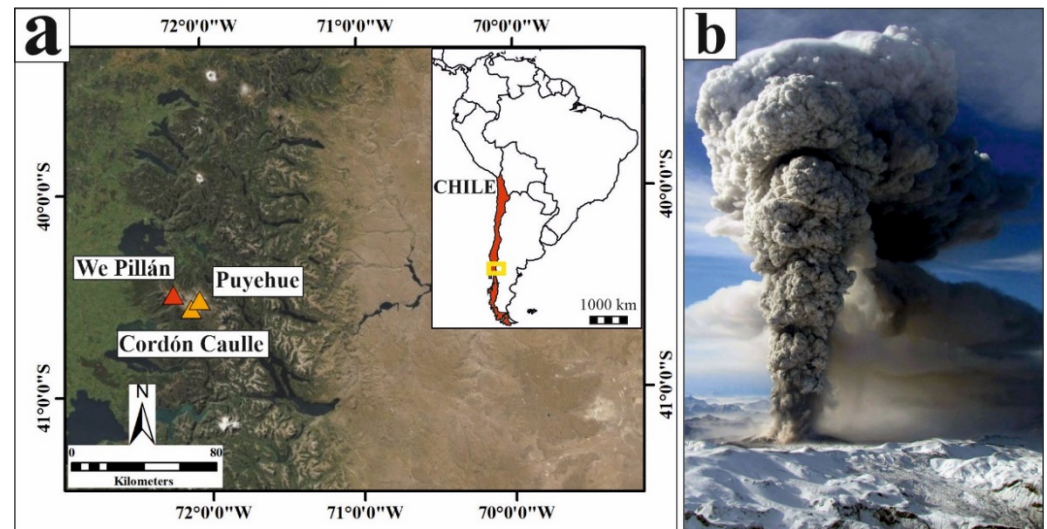
Figure 1. (a) Location of the Puyehue-Cordón Caulle complex and the We Pillán vent. Coordinates expressed in the WGS84 coordinate system. Service Layer Credits, courtesy of: Esri, DigitalGlobe, GeoEye, Earthstar Geographics, CNES/Airbus DS, USDA, USGS, AeroGRID, IGN, and the GIS User Community; (b) picture of the eruption on the 14 June 2011 (courtesy of Liz Keller; https://www.pinterest.com/pin/457537643392364548/ , accessed on 13 March 2021).
