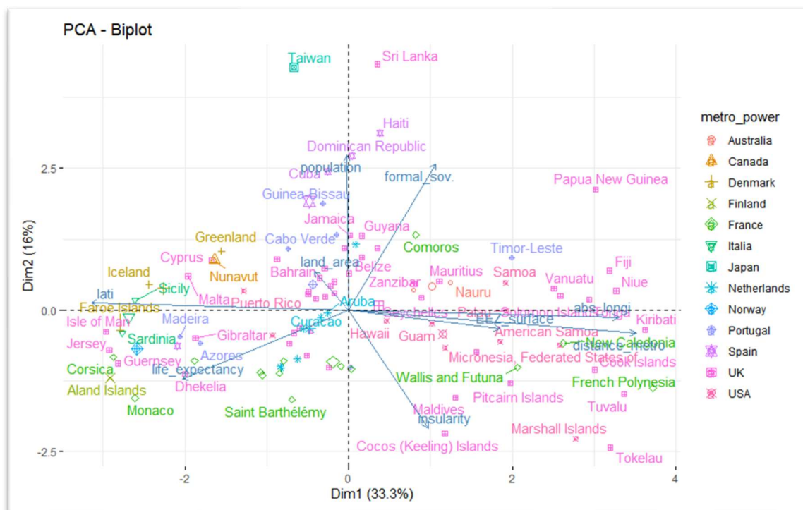
Figure 7: PCA contrasted with metropolitan powers.
