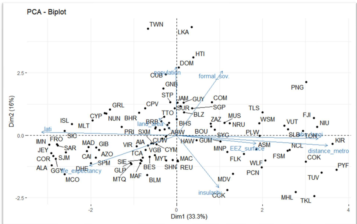
Figure 4: PCA results: location of the 100 SIEs.
