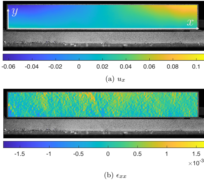
Fig. 11: Typical u_x displacement map and \epsilon_{xx} strain map obtained during milling after the 45th pass.
