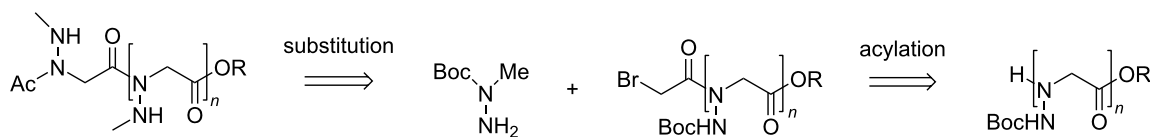
Figure 2: Solution-phase synthesis of N -(methylamino)glycine oligomers using N -Boc- N -methylhydrazine as a submonomer.
