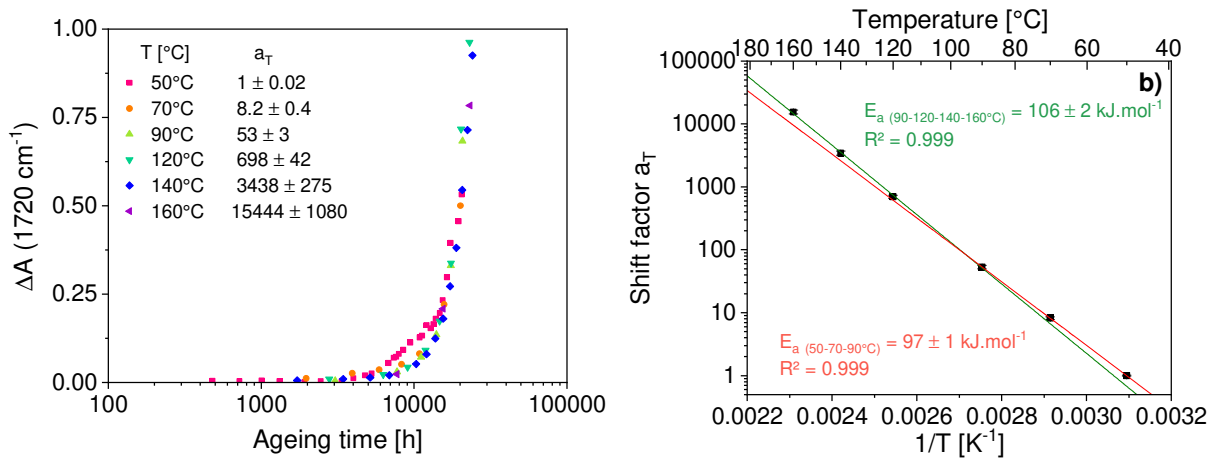
Figure 10: (a) Manual time-temperature superposition of the IR spectroscopic data of XLPE using T_{\text{ref}} = 50\text{ }^\circ\text{C} ; (b) Arrhenius plot of the shift factors a_T determined from spectroscopic data of XLPE using a manual time superposition in the range 50 - 160\text{ }^\circ\text{C} , with T_{\text{ref}} = 50\text{ }^\circ\text{C} .
