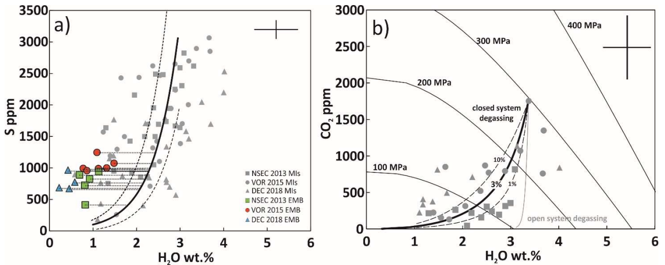
727 Figure 6. (a) Diagram reporting the average values of H 2 O-S compositions in the interior of the 728 embayments and the degassing model for the H 2 O-S system on MIs from the same eruptive episodes 729 (restored compositions for volatile loss; data from Zuccarello et al., 2021). Sulfur degassing has been 730 modeled by using the mass balance approach described in Spilliaert et al. (2006) (See supplementary 731 data for details). The thick black line is the best fit model, which is obtained starting from pressure 732 of 180 MPa, S = 3065 ppm and H 2 O = 2.9 wt.%, at melt fraction f = 85\% and initial gas phase \alpha_0 = 733 3%. Initial H 2 O concentrations before diffusive loss during ascent can be inferred from S degassing, 734 as well as the corresponding initial pressures are derived from the H 2 O-CO 2 system. The dashed lines 735 represent the \pm 1\sigma of S degassing model, while the thin dotted lines indicate the potential initial H 2 O 736 contents for each embayment (green squares: NSEC 2013; red circles: VOR 2015; blue triangles: 737 DEC 2018). (b) H 2 O-CO 2 closed degassing model on MIs from the same eruptive episodes 738 (Zuccarello et al., 2021). The thick black line is the intermediate path (with initial gas phase = 3%) 739 used for constraining initial pressures in the diffusion modeling for each embayment.
