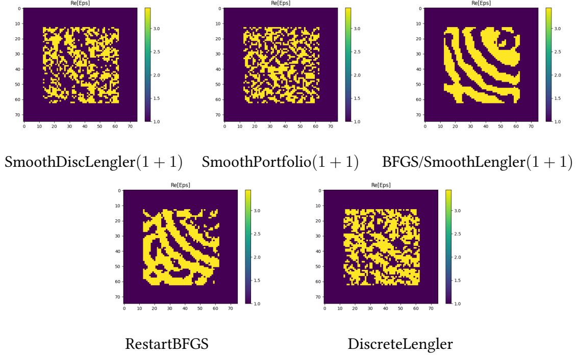
Figure 2: Visualization of waveguide bend designs with budget 3000, including smoothing operators. The light arrives from the middle at the top, and leaves at the middle on the right hand side.
