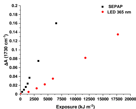
Fig. 6. Absorbance at 1730 cm -1 as a function of exposure in the SEPAP (irradiance 90 W m -2 ) and in the LED 365 setup (irradiance 82 W m -2 ).
