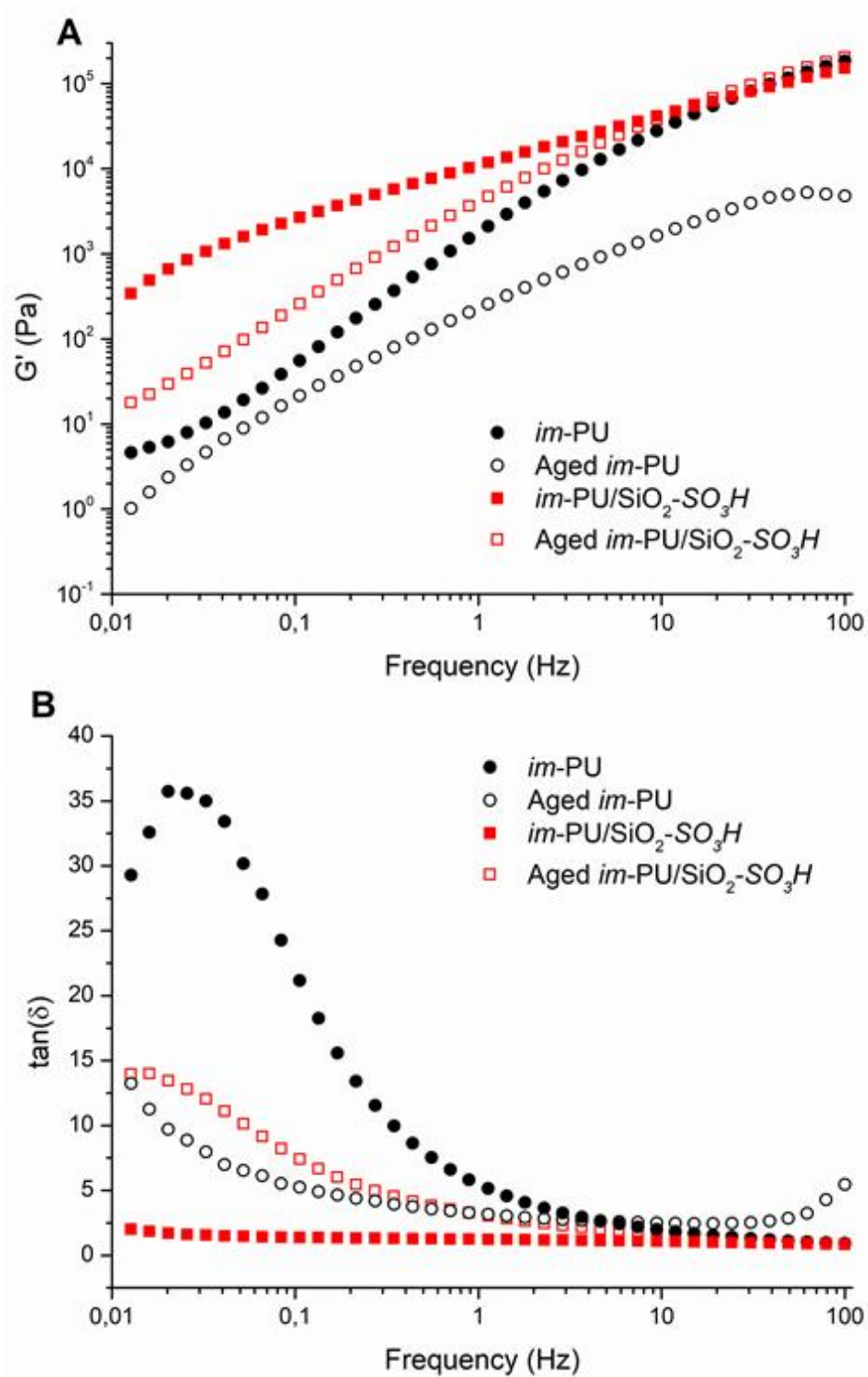
Figure 6. Storage modulus G' (A) and loss factor \text{Tan}\delta (B) of unaged im -PU (black, full circle), unaged ionic im -PU/SiO 2 -SO 3 H hybrid (red, full square), aged im -PU (black, open circle) and aged ionic im -PU/SiO 2 -SO 3 H hybrid (red, open square).
