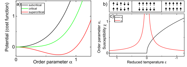
Figure 1: Illustration of the general theory of second-order phase transitions. a) Generalized potential F as a function of order parameter \alpha . The system always seeks to minimize F . The minimum is at \alpha = 0 "above" transition (subcritical behavior) and at \alpha \neq 0 "below" transition (supercritical behavior). b) Ising model of a ferromagnet illustrating the 3 regimes: subcritical (short correlations), critical (long-range dynamical correlations), supercritical (long-range static correlations). c) The order parameter \alpha , growing as a square root beyond the transition, and the susceptibility \chi , diverging at the critical point, as a function of a dimensionless parameter (reduced temperature \epsilon ).
