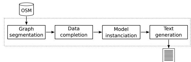
Figure 6. The processing pipeline from the OpenStreetMap data to the generated text.
