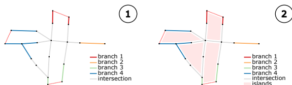
Figure 4. Steps for generating islands as presented in 3.3.2. Corresponding ways will contain the island's PedestrianNode.
