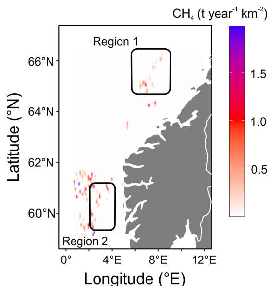
Figure 3. Spatially gridded \text{CH}_4 emissions from fuel exploitation for the northern North Sea and Norwegian Sea (Scarpelli et al., 2020). Regions surveyed in this study are represented by the boxes labelled “Region 1” and “Region 2”.
