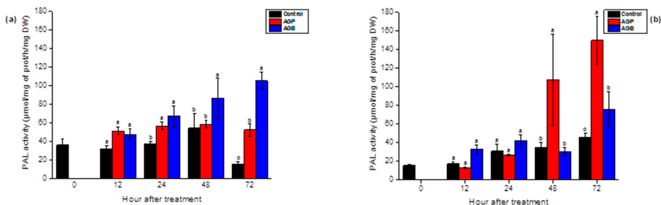
Figure 4. Stimulation of PAL activity in the leaves (a) and the roots (b) of tomato seedlings after injection (10 µL) of AGB and AGP fractions (1 g/L). Each value is the mean of four repetitions ± SE. The letters (a, b, o) indicate significant differences between treatments (Control, AGB, and AGP) in each point time using Tukey-HSD test, at ( p < 0.05 ). Treatments presented with the same letter are not significantly different.
