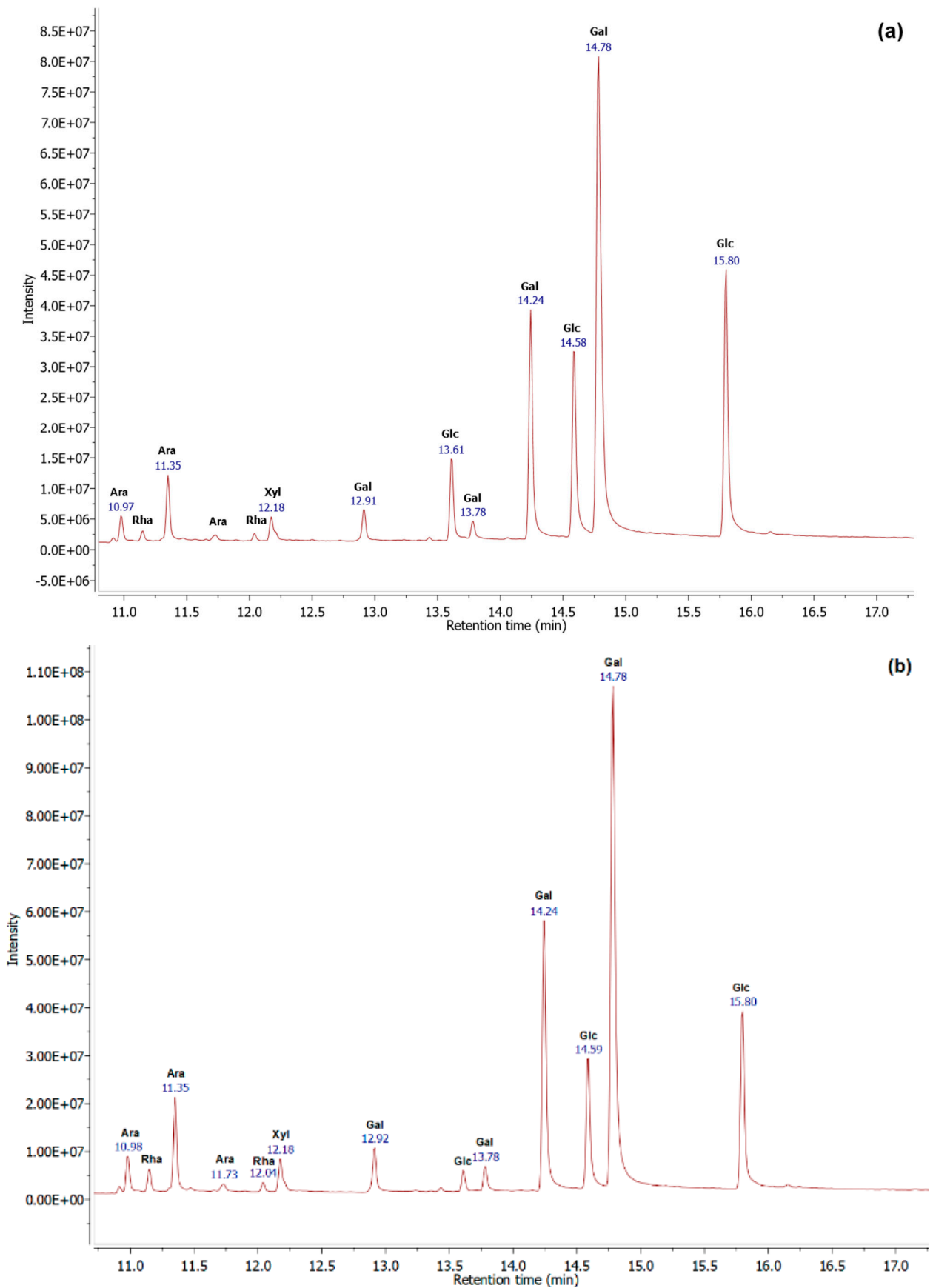
Figure 2. GC-EI/MS profiles of the sulfated glycoproteins AGB (a) and AGP (b), obtained using OPTIMA-1MS (30 m, 0.25 mm, 0.25 \mu m) column at a flow rate of 1.75 mL/min.
