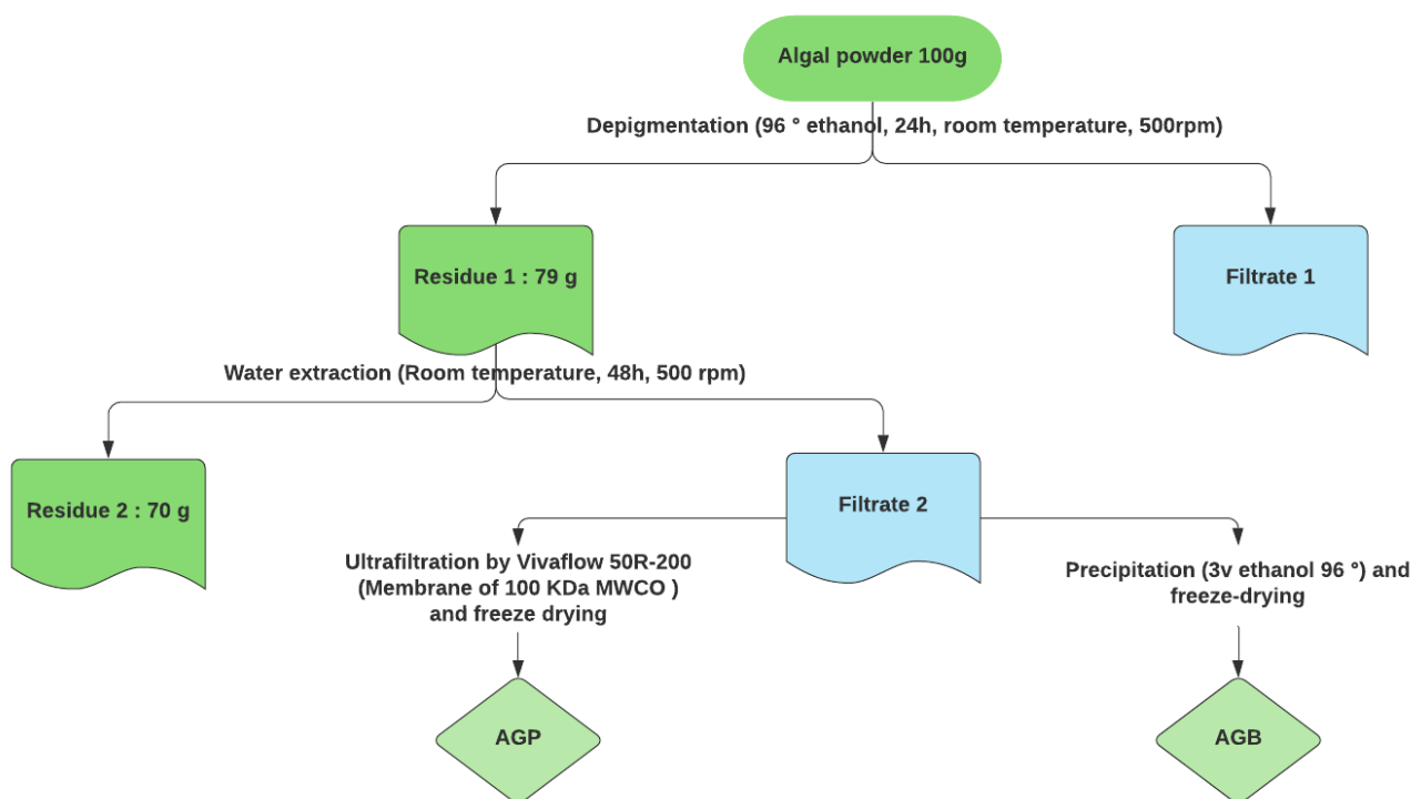
Figure 1. Process for extraction and purification of sulfated glycoproteins from C. decorticutum .
