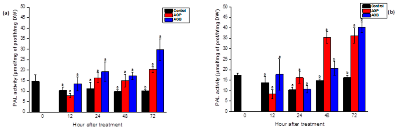
Figure 5. Stimulation of PAL activity in the leaves (a) and the roots (b) of tomato seedlings after foliar spray (20 mL) of AGB and AGP fractions (1 g/L). Each value is the mean of four repetitions ± SE. The letters (a, b) indicate significant differences between treatments (Control, AGB, and AGP) in each point time using a Tukey-HSD test at ( p < 0.05 ). Treatments presented with the same letter are not significantly different.
