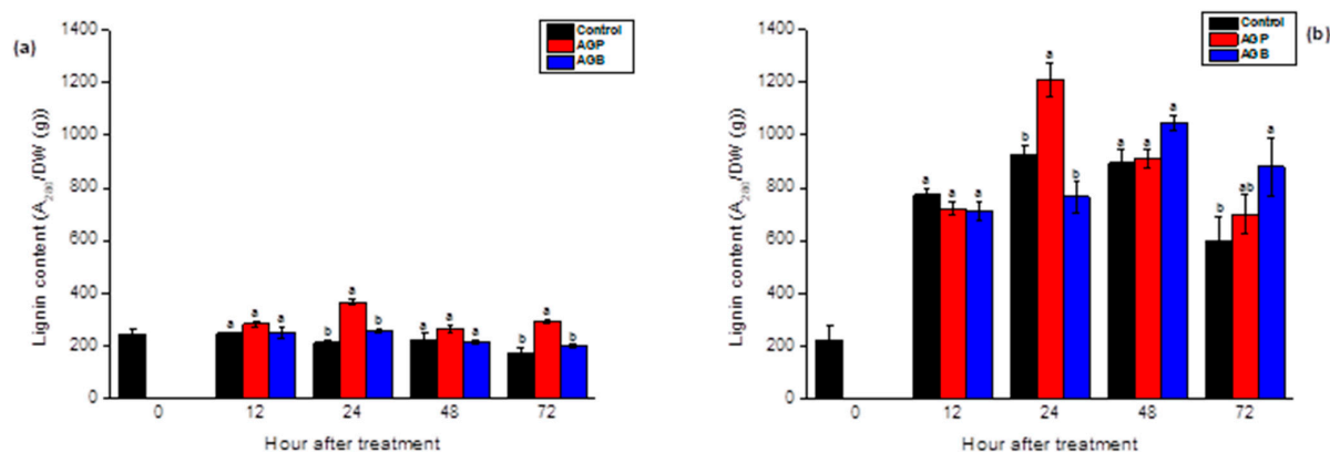
Figure 8. Lignin content in the leaves (a) and the roots (b) of tomato seedlings after injection (10 \mu L) of AGB and AGP fractions (1 g/L). Each value is the mean of four repetitions \pm SE. The letters (a, b) indicate significant differences between treatments (Control, AGB, and AGP) in each point time using the Tukey-HSD test, at ( p < 0.05 ). Treatments presented with the same letter are not significantly different.
