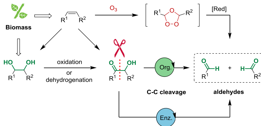
Scheme 1. Synthetic strategies for the preparation of aldehydes through C-C bond cleavage.
