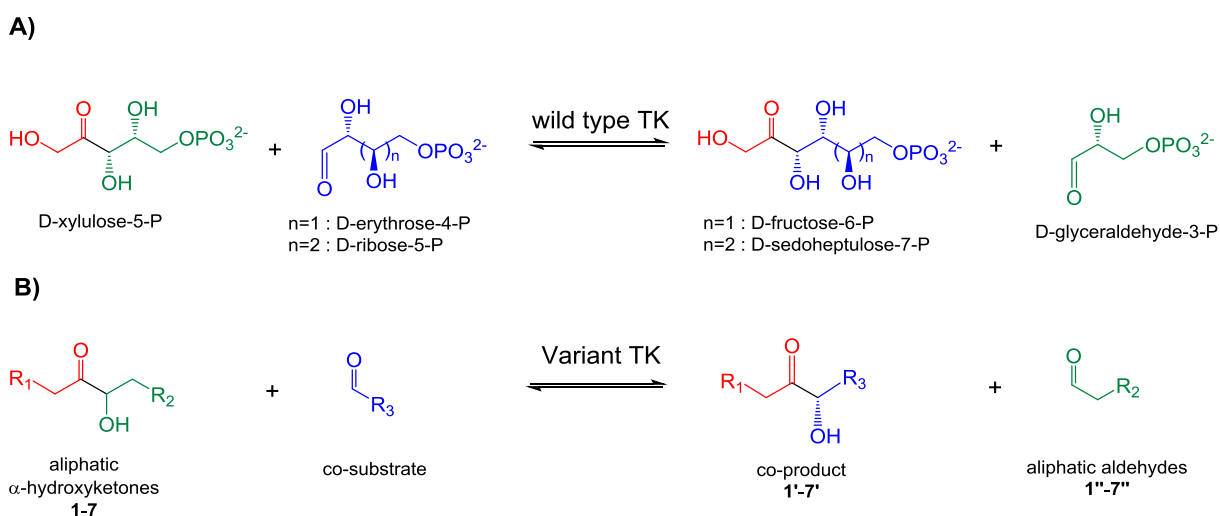
Scheme 2. TK-catalyzed reaction with wild type in the pentose phosphate pathway A) and with variants for in vitro \alpha -hydroxyketone cleavage B)
